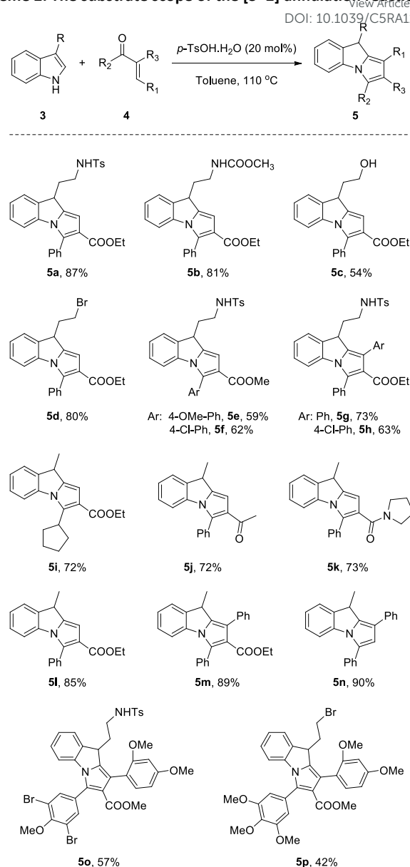
Scheme 2. The substrate scope of the [3+2] annulation reactions
