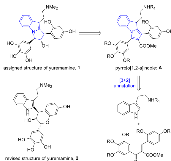
Scheme 1. Synthetic strategy toward the originally assigned structure of yuremamine
