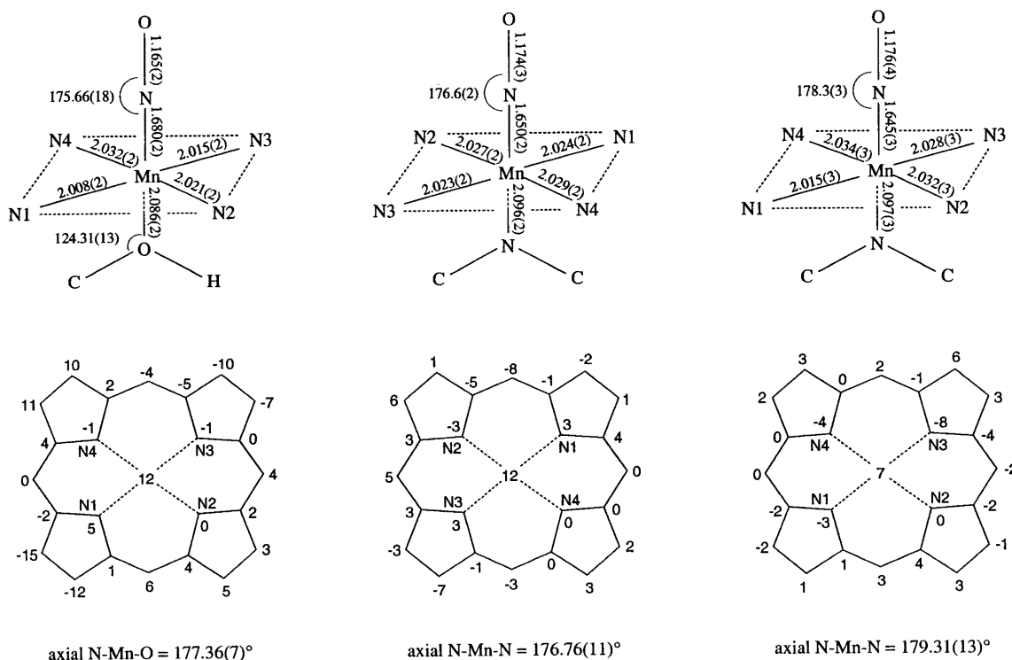
Fig. 3 Structural data for the ordered molecule of (TTP)Mn(NO)(CH 3 OH), the ordered molecule of (TTP)Mn(NO)(1-MeIm) and (T( p -OCH 3 )PP)Mn(NO)(1-MeIm). Selected bond lengths and angles are shown in the top sketches. Perpendicular atom displacements from the 24-atom porphyrin planes (in 0.01 Å units) are shown in the bottom sketches.
