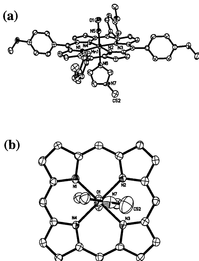
Fig. 2 (a) Molecular structure of (T( p -OCH 3 )PP)Mn(NO)(1-Melm). Hydrogen atoms have been omitted for clarity. (b) View of the orientation of the 1-Melm ligand relative to the porphyrin skeleton. The porphyrin p -methoxyphenyl substituents have been omitted for clarity.
