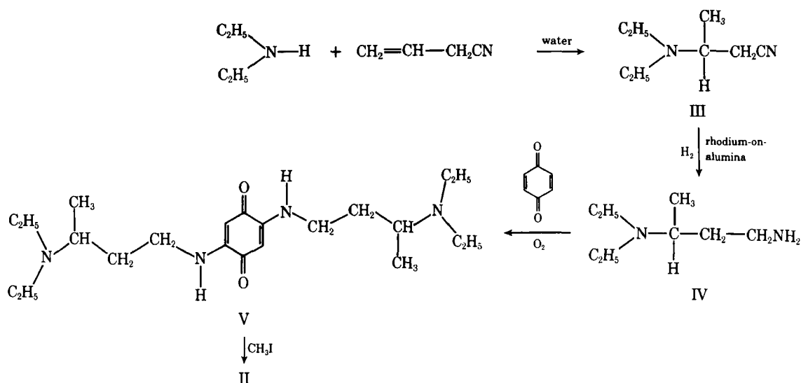
Scheme I—Synthetic route for preparation of II
