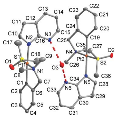
Fig. 7 ORTEP representation (50% probability) of the dimeric entity of 9 \cdot 0.5\text{H}_2\text{O} . The hydrogen atoms on O3 could not be found in this heavy atom structure. Distances and angles in Table 3; hydrogen bonding interaction as dashed line. Hydrogen atoms on carbon have been omitted for clarity.
