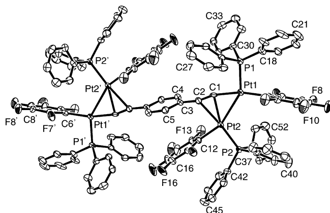
Figure 3. Molecular structure of [\{trans-(PPh_3)(C_6F_5)Pt(\mu-H)Pt(C_6F_5)(PPh_3)\}_2\{\mu-1\kappa C^\alpha:4\kappa C^{\alpha'}:\eta^2:\eta^2-(1,4-C\equiv C)_2-C_6H_4\}]\cdot 4CH_2Cl_2 ( 4a ·4CH 2 Cl 2 ). Ellipsoids are drawn at the 50% probability level. Hydrogen atoms have been omitted for clarity.
