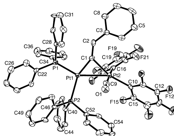
Figure 1. Molecular structure of [ cis,cis -(OC)(C 6 F 5 ) 2 Pt( \mu -1 \kappa C ^{\alpha} : 2 \kappa C ^{\alpha} -C=CHPh)Pt(PPh 3 ) 2 ] \cdot CHCl 3 \cdot C 6 H 14 ( 2 \cdot CHCl 3 \cdot C 6 H 14 ). Ellipsoids are drawn at the 50% probability level. Hydrogen atoms have been omitted for clarity.
