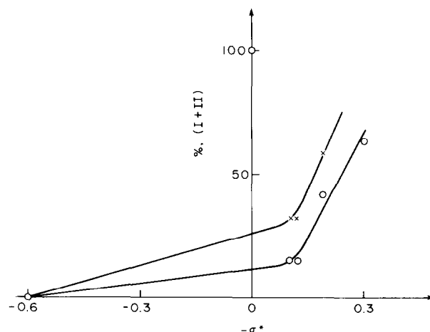
Fig. 3. The dependence of the summary yields of products I and II on the Taft constants \sigma^* of R ( R_2M , where M \equiv Zn (O) or Cd (X)) at 30°C.
