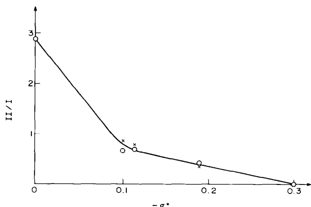
Fig. 4. The dependence of the ratio of product I and II yields on the Taft constants \sigma^* of R ( R_2M , where M \equiv \text{Zn} (○) or \text{Cd} (×)) at 0°C.
