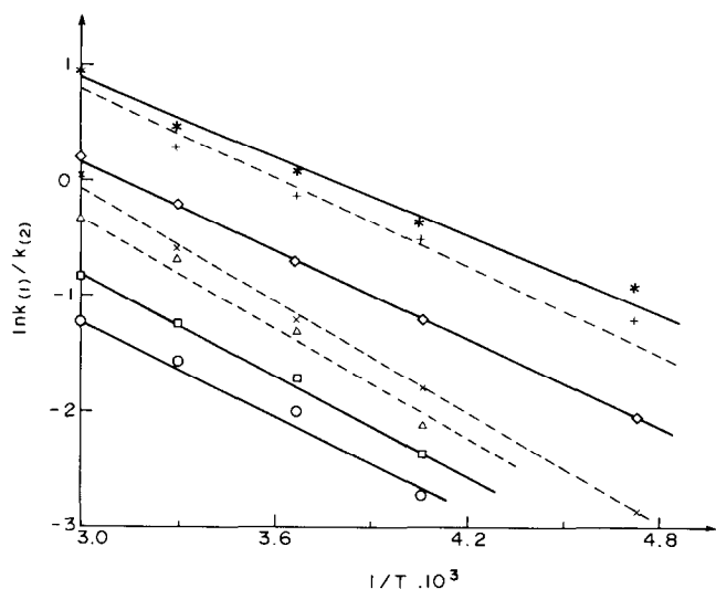
Fig. 2. The dependence of \ln(k_{(1)}/k_{(2)}) on 1/T in the reaction of 3,6-DTBQ with R_2M : \circ , Et_2Zn ; \square , nPr_2Zn ; \Delta , Et_2Cd ; \times , nPr_2Cd ; \diamond , iPr_2Zn ; + , iPr_2Cd ; * , tBu_2Zn .
