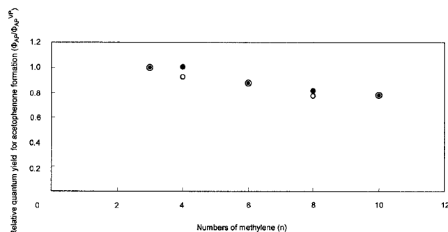
Figure 2. Relative quantum yields for production of acetophenone from alkyl phenyl ketones \text{PhCO}(\text{CH}_2)_n\text{CH}_3 in benzene containing 0.5 M pyridine (○) and on a silica-gel surface (●)
