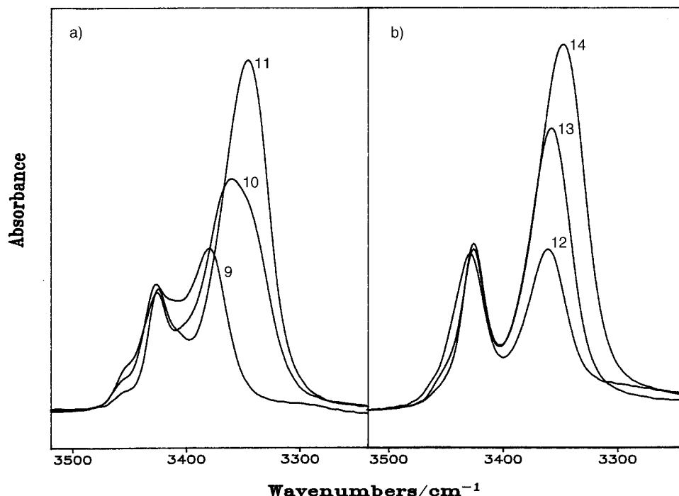
Fig. 4. FT-IR Absorption spectra (3500–3200-cm -1 region) in CDCl 3 solution of a) Z-(S)-Bin-(Aib) 2 -O t Bu ( 9 ), Z-(S)-Bin-(Aib) 2 -(S)-Bin-O t Bu ( 10 ), and Z-(S)-Bin-(Aib) 2 -(S)-Bin-Aib-O t Bu ( 11 ); b) Z-(Aib) 2 -(S)-Bin-O t Bu ( 12 ), Z-(Aib) 2 -(S)-Bin-Aib-O t Bu ( 13 ), and Z-(Aib) 2 -(S)-Bin-(Aib) 2 -O t Bu ( 14 ). Peptide concentration 1.0 mM
