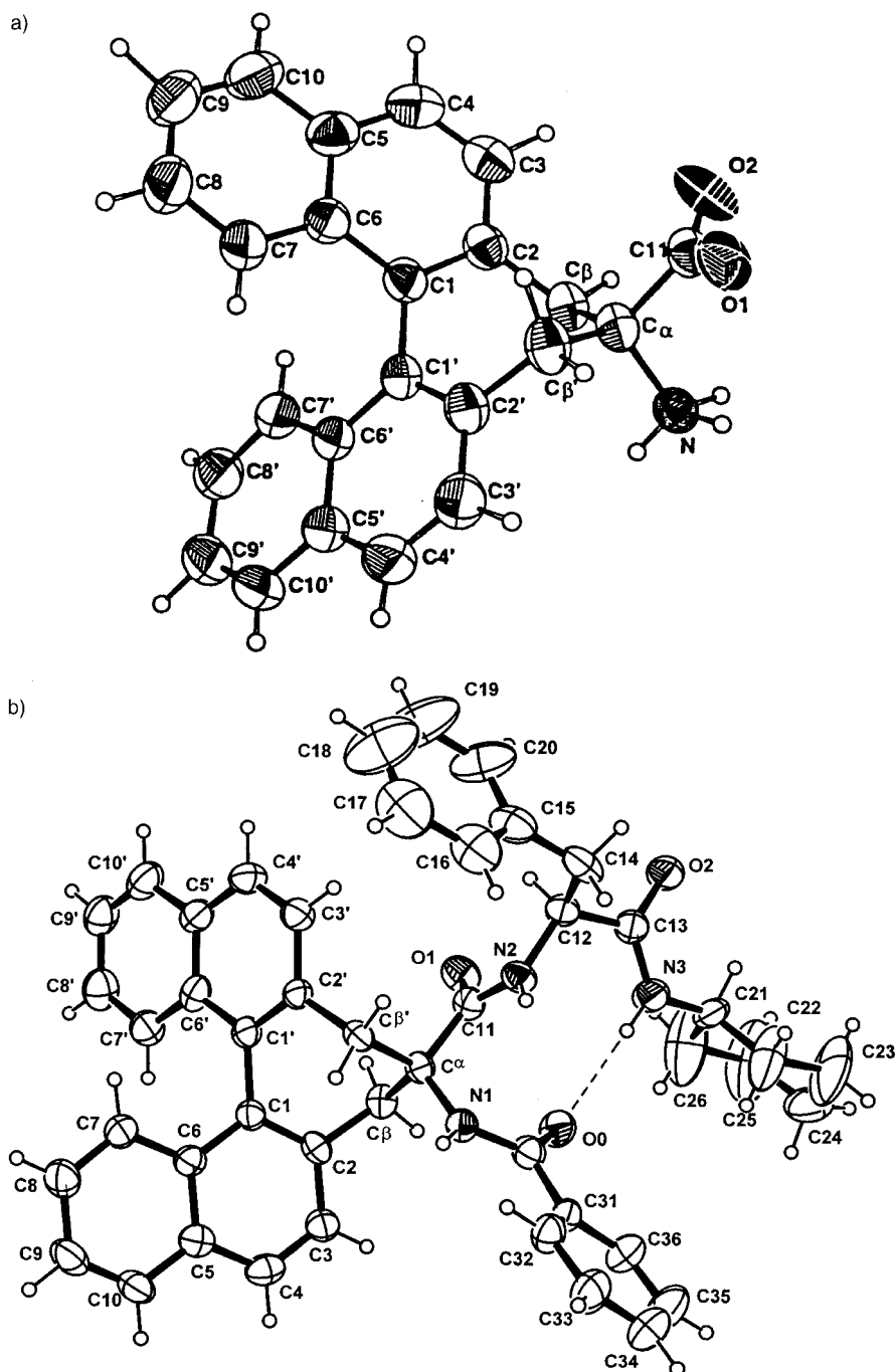
Fig. 7. X-Ray diffraction structures of a) H^+ \cdot H-(S)\text{-Bin-O}^- and b) Bz-(R)\text{-Bin-Phe-NHChx} ( 1' ) with numbering of the atoms. The C=O \cdots H-N intramolecular H-bond is indicated by a dashed line. Arbitrary numbering.
