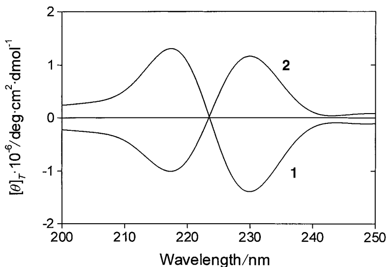
Fig. 2. CD Spectra in the 200–250-nm region of Ac-(R)-Bin-Phe-NHChx ( 1 ) and Ac-(S)-Bin-Phe-NHChx ( 2 ) in MeOH solution. Peptide concentration, 1.0 mM.
