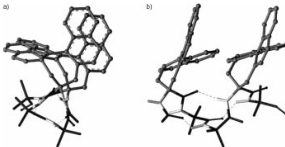
Fig. 6. Molecular model of the 3_{10} -helical structure formed by the \text{N}^\alpha -acylated pentapeptide sequence -(\text{S})\text{-Bin}-(\text{Aib})_2-(\text{S})\text{-Bin-Aib}- of 11 . a) Top view; b) side view.
