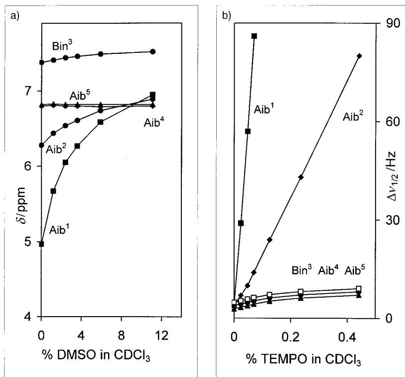
Fig. 5. a) Plot of NH chemical shifts in the ^1\text{H} -NMR spectrum of \text{Z}-(\text{Aib})_2-(\text{S})\text{-Bin}-(\text{Aib})_2-\text{O}^t\text{Bu} ( 14 ) as a function of increasing percentages of DMSO added to the \text{CDCl}_3 solution (v/v). b) Plot of bandwidths of the NH signals in the ^1\text{H} -NMR spectrum of 14 as a function of increasing percentages of TEMPO (w/v) added to the \text{CDCl}_3 solution. Peptide concentration, 1.0 mM.
