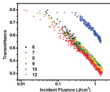
Figure 11. Transmission vs incident fluence curves for 6–10 and 12 in \text{CH}_2\text{Cl}_2 solutions for 4.1 ns laser pulses at 532 nm in a 2 mm cell. The linear transmission was adjusted to 80%.
