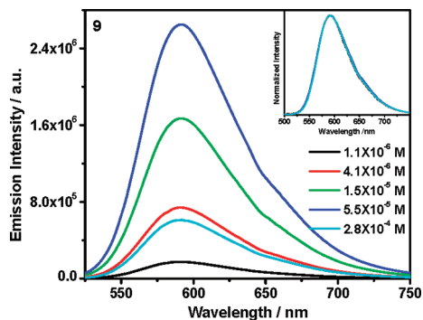
Figure 7. Emission spectra of complex 9 in degassed CH 2 Cl 2 solutions at different concentrations at room temperature.
