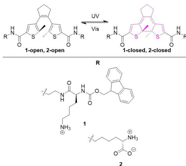
Fig. 1 Photoisomerization of DTE photochromic unit and structures of DTE bolaamphiphile 1 .
