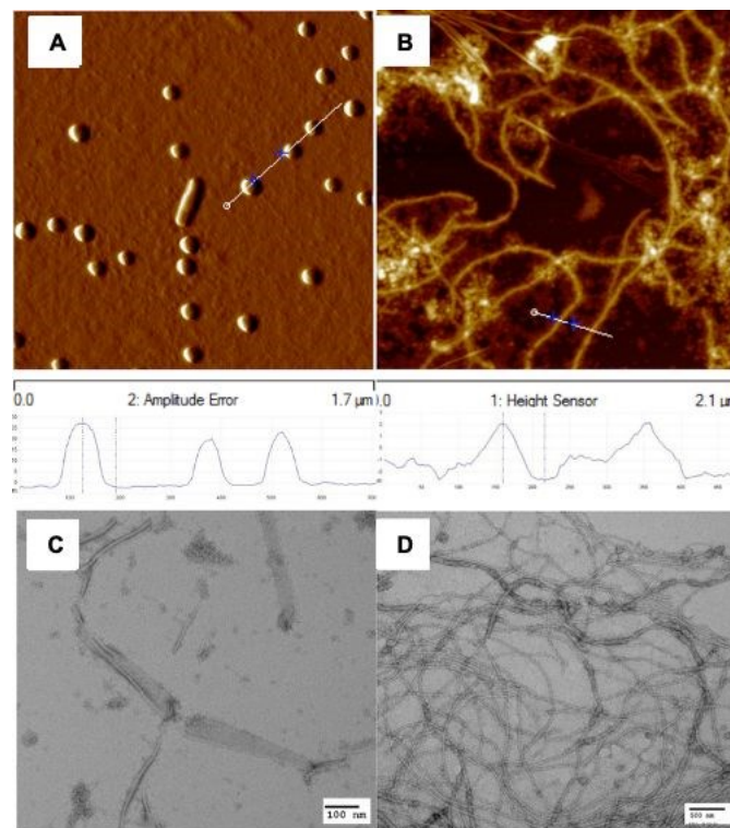
Fig. 2: Tapping-mode AFM images of 1 (A) in the open state and, (B) 24 h after irradiation in water with 254 nm light. (C) TEM images of 1 after exposure to 254 nm light and subsequent aging for 0 h and (D) 24 h. Samples were prepared by dissolving 1 in water (10 mM), prior to diluting to 500 \mu M (TEM) and evaporating onto a carbon-coated copper grid with uranyl acetate as a negative stain (TEM) or diluting to 100 \mu M and evaporating onto freshly cleaved mica (AFM).
