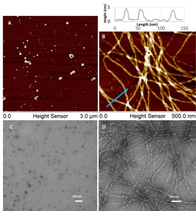
Fig. 4 Tapping-mode AFM (top) and TEM (bottom) images of 1 : (A/C) 1-open (10 mM) and (B/D) 1-closed . Samples of 1-closed were prepared by irradiation with 254 nm light in methanol for ~40 min (for 1-closed ), evaporation and redissolution in water (10 mM), sonication (20% amp., 5 min., pulsed) and aging for 24 h in darkness. AFM and TEM images were recorded after diluting in water (1 mM) and evaporating onto a carbon-coated copper grid with 2% aq. uranyl acetate as a negative stain (TEM) or onto freshly cleaved mica (AFM).
