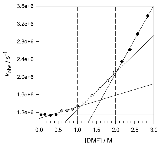
Figure 2. Plot of the observed rate constant ( k_{\text{obs}} ) against [\text{DMF}] for reaction of the cumyloxyl radical ( \text{CumO}^\bullet ) measured at T = 25^\circ \text{C} in an argon-saturated acetonitrile solution containing 1.0 M dicumyl peroxide and 0.5 M \text{LiOTf} , following 355 nm LFP. From the linear regression analysis in the 0.5–1.0 M [\text{DMF}] range (gray circles), k_{\text{H1}} = 2.62 \times 10^5 \text{ M}^{-1} \text{ s}^{-1} , r^2 = 0.89 ; in the 1.0–2.0 M [\text{DMF}] range (white circles), k_{\text{H2}} = 8.41 \times 10^5 \text{ M}^{-1} \text{ s}^{-1} , r^2 = 0.9934 ; in the 2.0–2.7 M [\text{DMF}] range (black diamonds), k_{\text{H3}} = 1.54 \times 10^6 \text{ M}^{-1} \text{ s}^{-1} , r^2 = 0.9970 . The dashed lines highlight [\text{DMF}] of 1.0 and 2.0 M.
