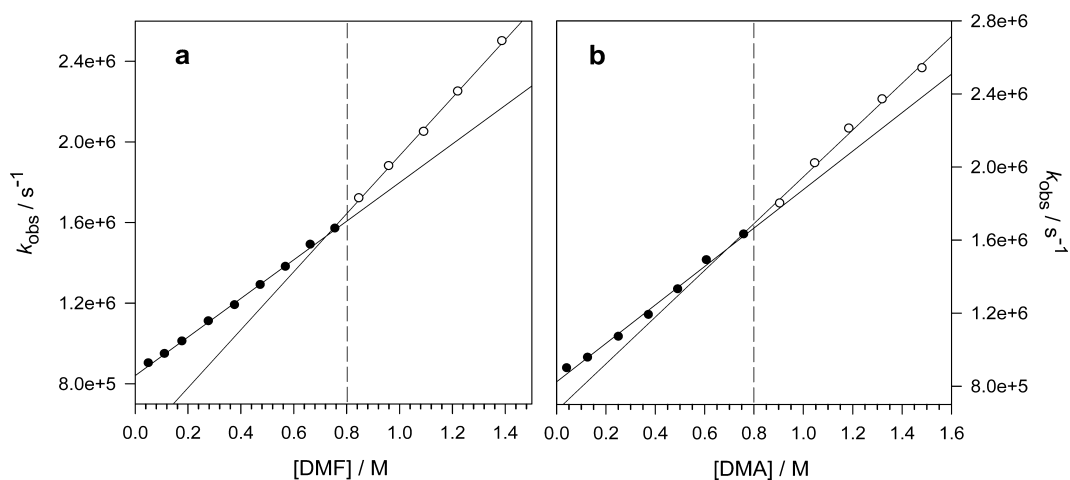
Figure 3. (a) Plot of the observed rate constant ( k_{\text{obs}} ) against [DMF] for reaction of the cumyloxy radical ( \text{CumO}^\bullet ) measured at T = 25^\circ\text{C} in an argon-saturated acetonitrile solution containing 1.0 M dicumyl peroxide and 0.2 M \text{NaClO}_4 , following 355 nm LFP. From the linear regression analysis in the 0–0.8 M [DMF] range (black circles), k_{\text{H1}} = 9.58 \times 10^5 \text{ M}^{-1} \text{ s}^{-1} , r^2 = 0.9987 ; in the 0.8–1.4 M [DMF] range (white circles), k_{\text{H2}} = 1.44 \times 10^6 \text{ M}^{-1} \text{ s}^{-1} , r^2 = 0.9990 . The dashed line highlights [DMF] of 0.8 M. (b) Plot of the observed rate constant ( k_{\text{obs}} ) against [DMA] for reaction of the cumyloxy radical ( \text{CumO}^\bullet ) measured at T = 25^\circ\text{C} in an argon-saturated acetonitrile solution containing 1.0 M dicumyl peroxide and 0.2 M \text{NaClO}_4 , following 355 nm LFP. From the linear regression analysis in the 0–0.8 M [DMA] range (black circles), k_{\text{H1}} = 1.05 \times 10^6 \text{ M}^{-1} \text{ s}^{-1} , r^2 = 0.9938 ; in the 0.8–1.5 M [DMA] range (white circles), k_{\text{H2}} = 1.28 \times 10^6 \text{ M}^{-1} \text{ s}^{-1} , r^2 = 0.9933 . The dashed line highlights [DMA] of 0.8 M.
