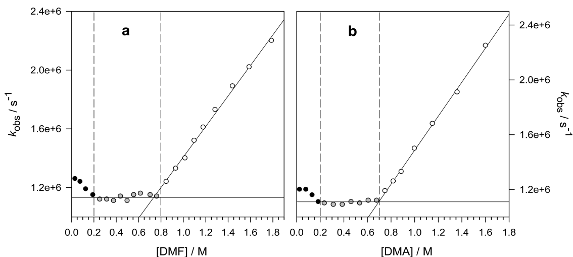
Figure 6. (a) Plot of the observed rate constant ( k_{\text{obs}} ) against [DMF] for reaction of the cumyloxyl radical ( \text{CumO}^\bullet ) measured at T = 25^\circ \text{C} in an argon-saturated acetonitrile solution containing 1.0 M dicumyl peroxide and 0.2 M \text{Ca}(\text{ClO}_4)_2 , following 355 nm LFP. From the linear regression analysis in the 0.8–1.8 M [DMF] range (white circles), k_{\text{H1}} = 1.04 \times 10^6 \text{ M}^{-1} \text{ s}^{-1} , r^2 = 0.9963 . The dashed lines highlight [DMF] of 0.2 and 0.8 M. (b) Plot of the observed rate constant ( k_{\text{obs}} ) against [DMA] for reaction of the cumyloxyl radical ( \text{CumO}^\bullet ) measured at T = 25^\circ \text{C} in an argon-saturated acetonitrile solution containing 1.0 M dicumyl peroxide and 0.2 M \text{Ca}(\text{ClO}_4)_2 , following 355 nm LFP. From the linear regression analysis in the 0.7–1.6 M [DMA] range (white circles), k_{\text{H1}} = 1.24 \times 10^6 \text{ M}^{-1} \text{ s}^{-1} , r^2 = 0.9982 . The dashed lines highlight [DMA] of 0.2 and 0.7 M.
