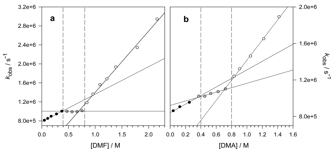
Figure 4. (a) Plot of the observed rate constant ( k_{\text{obs}} ) against [DMF] for reaction of the cumyloxy radical ( \text{CumO}^\bullet ) measured at T = 25^\circ\text{C} in an argon-saturated acetonitrile solution containing 1.0 M dicumyl peroxide and 0.2 M \text{Mg}(\text{ClO}_4)_2 , following 355 nm LFP. From the linear regression analysis in the 0–0.4 M [DMF] range (black circles), k_{\text{H1}} = 5.79 \times 10^5 \text{ M}^{-1} \text{ s}^{-1} , r^2 = 0.9965 ; in the 0.8–2.2 M [DMF] range (white circles), k_{\text{H2}} = 1.29 \times 10^6 \text{ M}^{-1} \text{ s}^{-1} , r^2 = 0.9950 . The dashed lines highlight [DMF] of 0.4 and 0.8 M. (b) Plot of the observed rate constant ( k_{\text{obs}} ) against [DMA] for reaction of the cumyloxy radical ( \text{CumO}^\bullet ) measured at T = 25^\circ\text{C} in an argon-saturated acetonitrile solution containing 1.0 M dicumyl peroxide and 0.2 M \text{Mg}(\text{ClO}_4)_2 , following 355 nm LFP. From the linear regression analysis in the 0–0.4 M [DMA] range (black circles), k_{\text{H1}} = 4.69 \times 10^5 \text{ M}^{-1} \text{ s}^{-1} , r^2 = 0.9951 ; in the 0.4–0.8 M [DMA] range (gray circles), k_{\text{H2}} = 2.43 \times 10^5 \text{ M}^{-1} \text{ s}^{-1} , r^2 = 0.96 ; in the 0.8–1.4 M [DMA] range (white circles), k_{\text{H3}} = 1.11 \times 10^6 \text{ M}^{-1} \text{ s}^{-1} , r^2 = 0.9988 . The dashed lines highlight [DMA] of 0.4 and 0.8 M.
