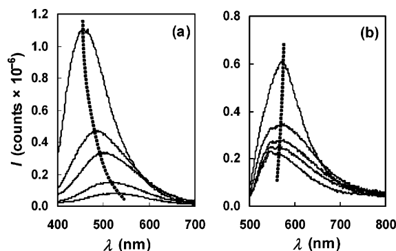
Figure 6. Photoexcitation and -emission spectra for 2 \mu M solutions of complex 4a in \text{CH}_2\text{Cl}_2/\text{MeCN} mixtures in order of decreasing intensity: 100:0 (neat \text{CH}_2\text{Cl}_2 ); 80:20; 50:50; 20:80; 0:100 (neat MeCN): (a) higher energy ^1\text{TICT} emission; (b) lower energy ^1\text{d}_\text{W}-\pi^*\text{W}=\text{CAr} emission.
