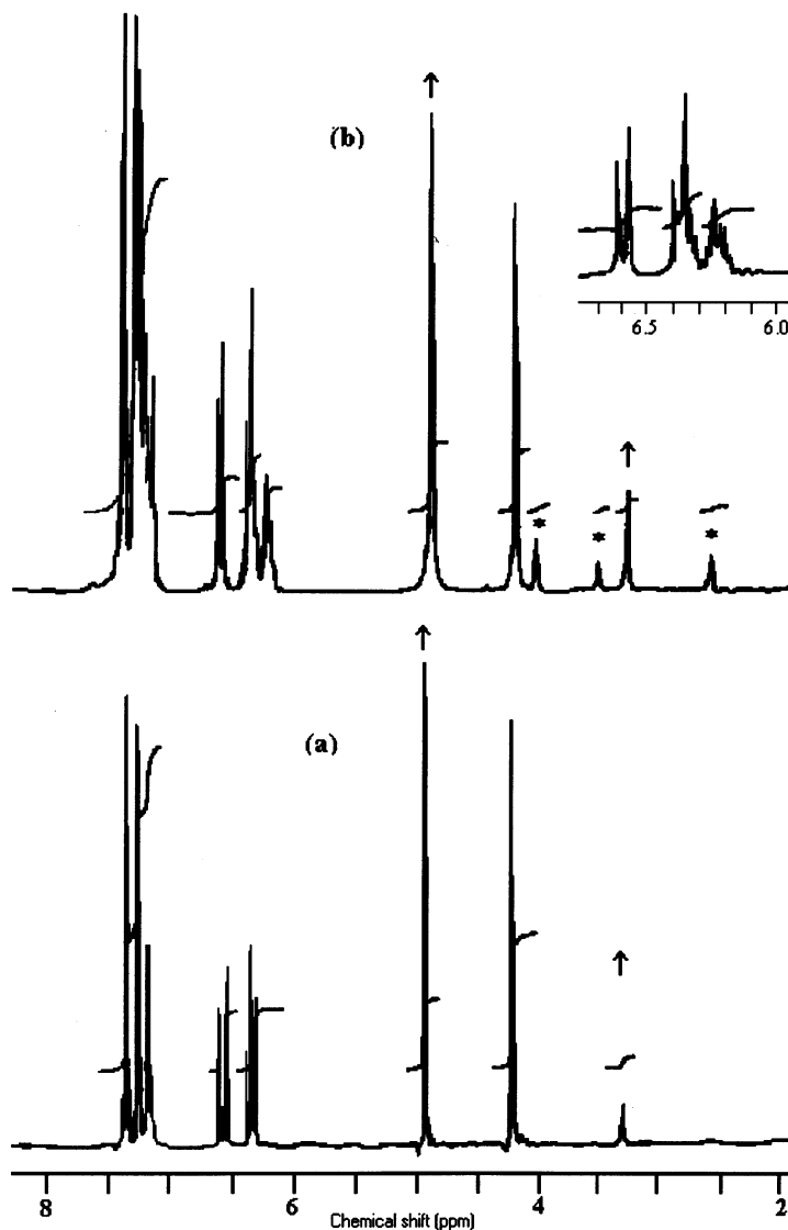
Fig. 1. The 400 MHz ^1\text{H} -NMR of the reaction mixture of trans -3-phenyl-2-propenal with sodium borohydride in \text{CD}_3\text{OD} (a) without \text{Ni}(\text{bpy})\text{Cl}_2 catalyst; (b) with \text{Ni}(\text{bpy})\text{Cl}_2 catalyst (* are signals from the saturated alcohol and \uparrow are from the solvent). Inset is the expansion of \alpha and \beta -proton signals of (b).
