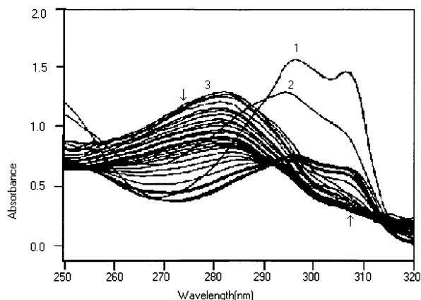
Fig. 2. Change of absorbance spectra of a methanolic solution containing \text{Ni}(\text{bpy})\text{Cl}_2 (0.023 mmol) with sodium borohydride (0.05 mmol) after 2 min time intervals.
