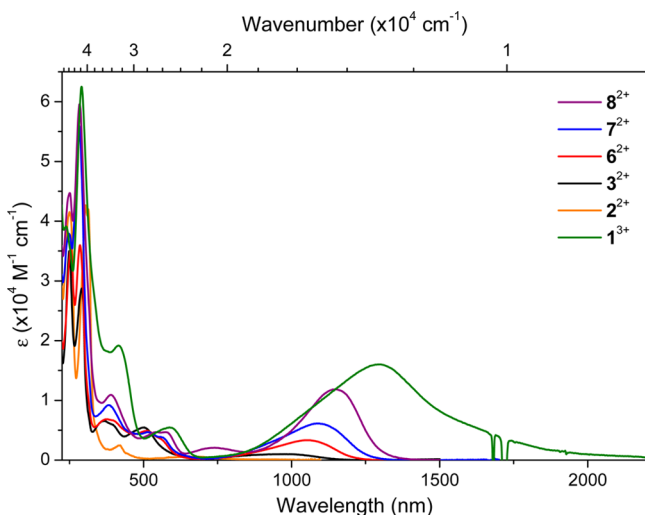
Figure 12. Overlay of UV-vis-NIR electronic absorption data recorded following controlled potential electrolysis of 1^{3+} and complexes 2^{2+} , 3^{2+} , 6^{2+} , 7^{2+} , and 8^{2+} in 0.1 M \text{Bu}_4\text{NPF}_6 acetonitrile electrolyte.
