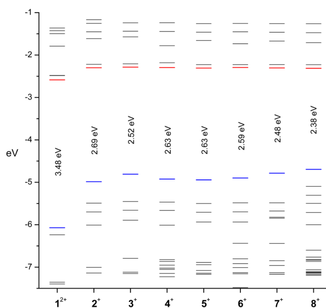
Figure 4. Plot of molecular orbital energy levels (eV) for complexes 1^{2+} – 8^+ as calculated by DFT/B3LYP/6-31g(d,p) (C,H,N,O) and LANL08 (Ru) in an acetonitrile solvent continuum model. Electron occupancy is removed for clarity, and HOMO and LUMO levels are highlighted in blue and red, respectively.
