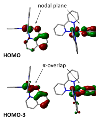
Figure 2. Aerial and side-on perspective views of both the HOMO and HOMO – 3 levels for 2^+ illustrating the \pi -bonding/antibonding combination of \text{Ru}(d\pi) and \text{OQN}(\pi) systems. For complete DFT results please refer to the Supporting Information. An acetonitrile polarizable continuum model was employed using the B3LYP functional and 6-31g(d,p) (C,H,N,O) and LANL08 (Ru) basis sets.
