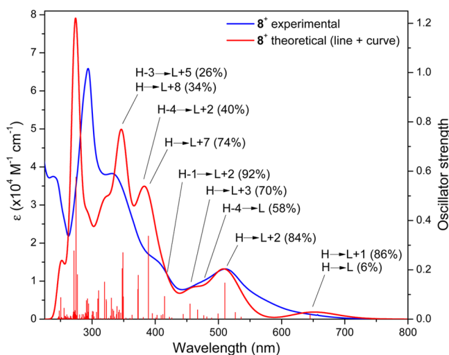
Figure 6. Overlay of experimental and theoretical TD-DFT spectra for 8^+ in acetonitrile. An acetonitrile polarizable continuum model was employed using the B3LYP functional and 6-31g(d,p) ( \text{C,H,N,O} ) and LANL08 (Ru) basis sets.
