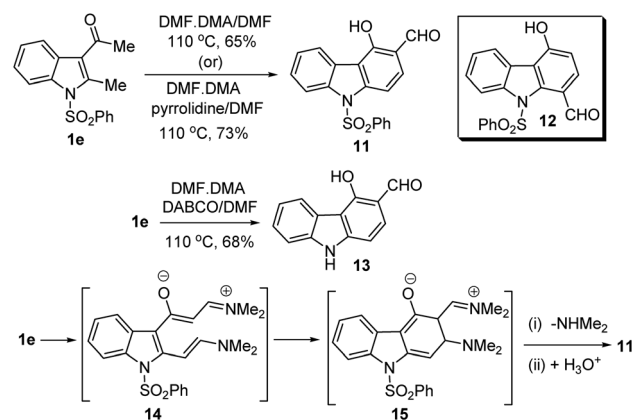
Scheme 5. Tandem reaction of 2-methyl-3-acetylindole 1e with DMF-DMA.
