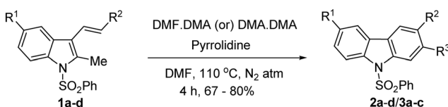
Scheme 2. Tandem reaction of 2-methylindoles 1a–d with DMF-DMA/DMA-DMA in the presence of pyrrolidine.
