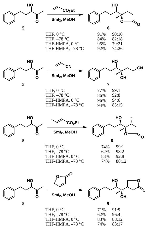
Scheme 2. \text{SmI}_2 -induced reductive coupling of 5 with various radical receptors.
