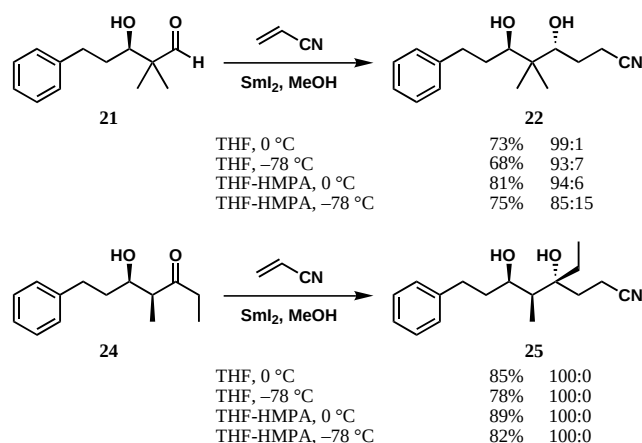
Scheme 4. Diastereoselectivities achieved in the reductive couplings of 21 and 24 with \text{SmI}_2 .
