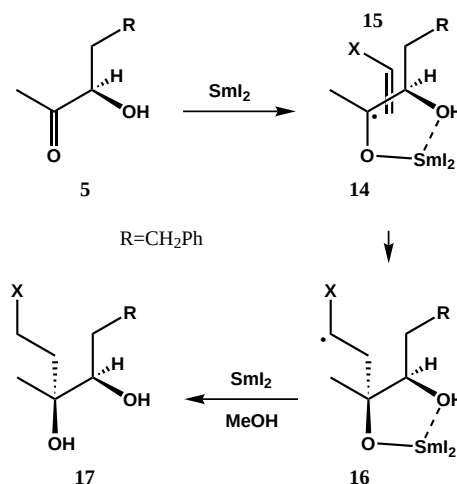
Scheme 3. Chelation-control model.
