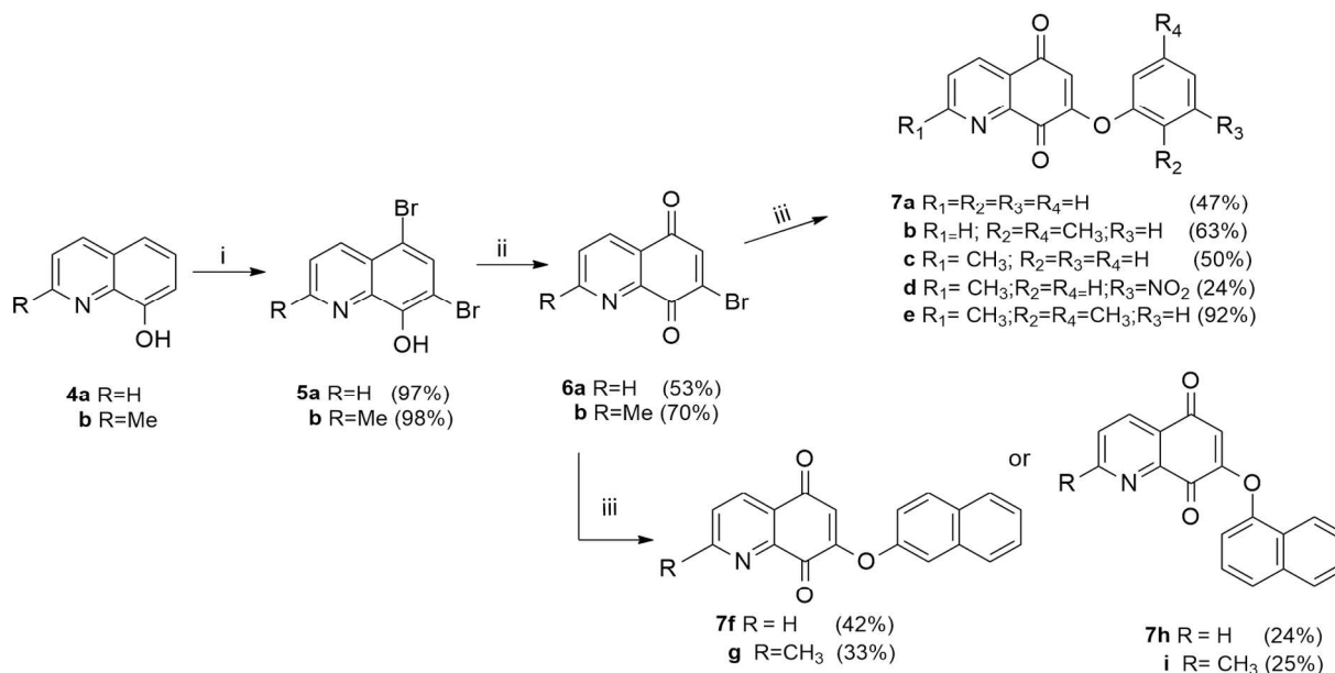
Scheme 2. Synthesis of compounds of series II ( 7a-i ). Reagents and conditions: (i) Br 2 , MeOH, rt, 5 min; (ii) HNO 3 , H 2 SO 4 , 0 °C, 30 min; 23 (iii) K 2 CO 3 , 2a-e , DMF, rt, 3-5 h.
