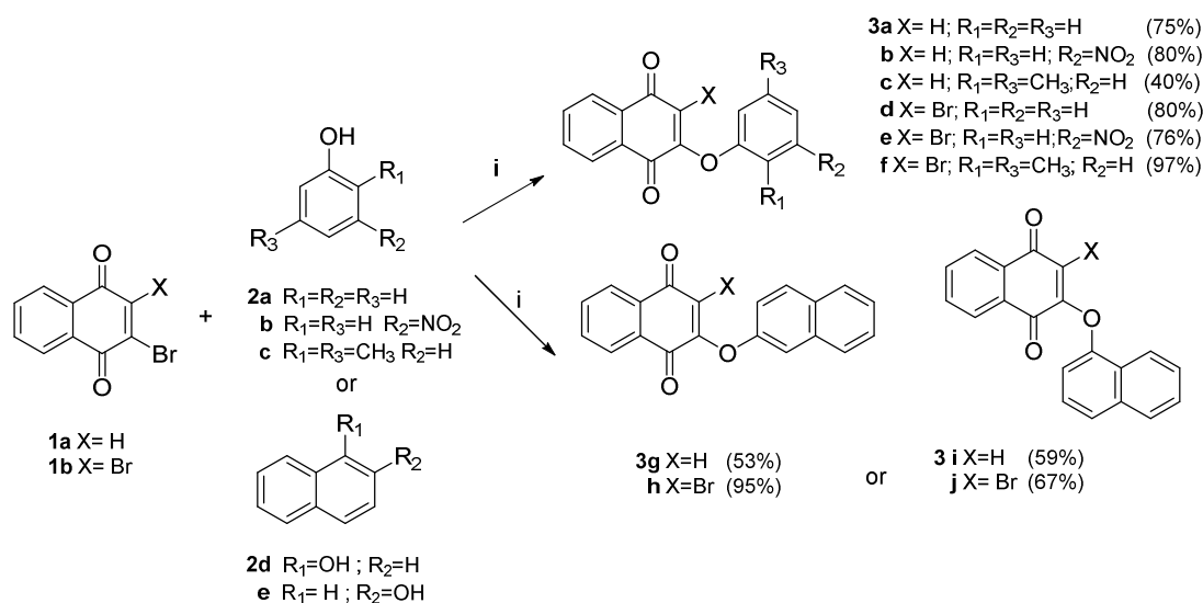
Scheme 1. Synthesis of compounds of series I ( 3a-j ). Reagents and conditions: (i) K 2 CO 3 , DMF, rt, 2-3 h.
