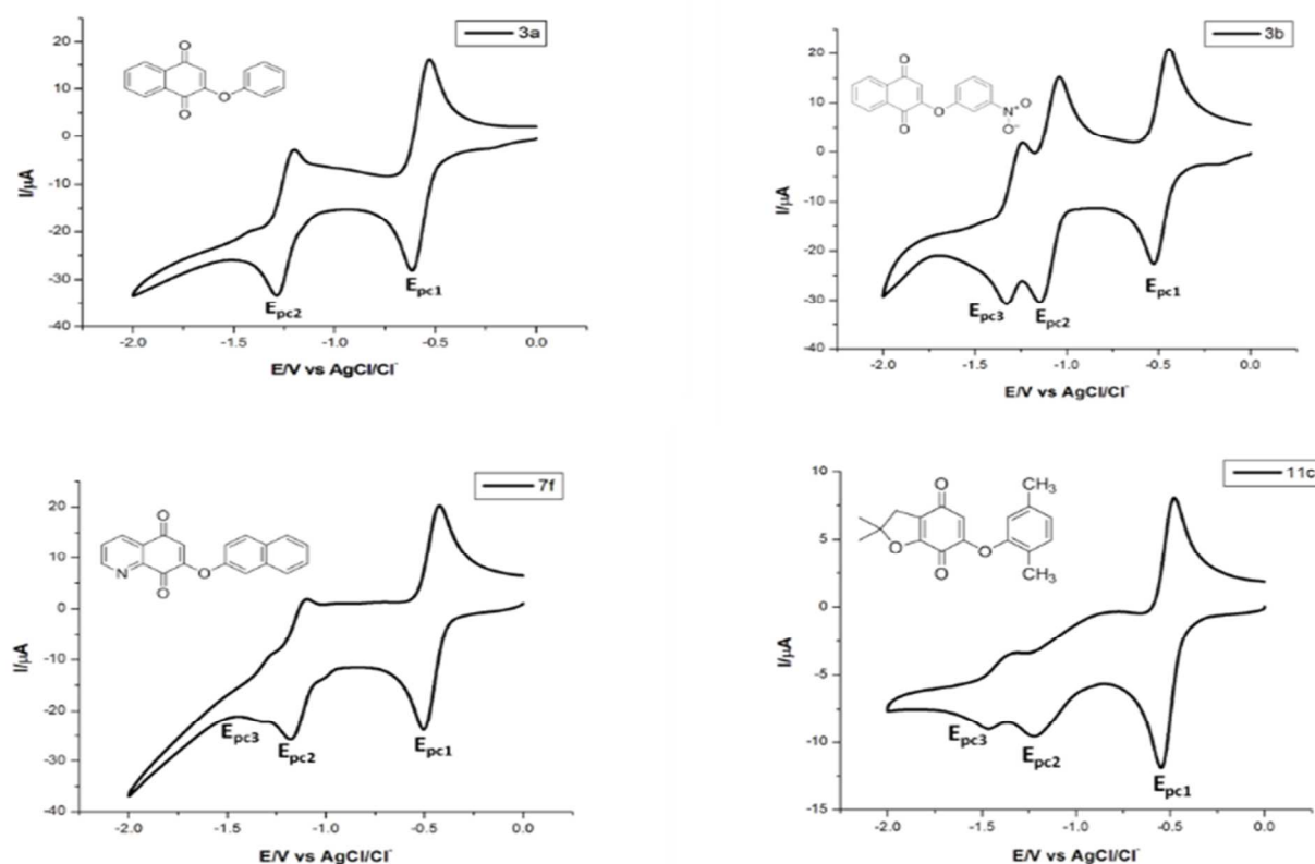
Fig. 4 Cyclic voltammograms of quinones 3a , 3b , 7f and 11c (1.0 mM). DMF/TBAP (0.1 M), glassy carbon electrode, cathodic direction, scan rate 50 mV s -1 .
