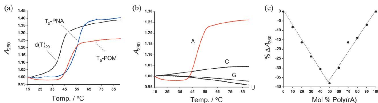
Fig. 5 (a) UV thermal denaturation curves of Phth-T 5 -POM 35, Lys-T 5 -LysNH 2 -PNA ( N - and C -terminal Lys, with C -terminal amide) and d(T) 20 vs. poly(rA) (42 μM each in bases) in buffer A (10 mM K 2 HPO 4 ) adjusted to 0.12 M K + , pH 7.0. (b) UV thermal denaturation curves for Phth-T 5 -POM 35 and an equimolar amount (42 μM each strand in bases) of poly(rA), (rU), (rC) or (rG) in buffer A adjusted to 0.12 M K + , pH 7.0. (c) A Job plot of the % change in A 260 vs. molar ratio Phth-T 5 -POM 35 and poly(rA).
