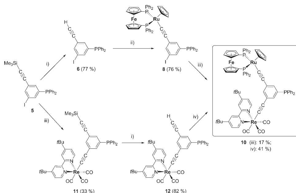
Scheme 2. Synthesis of trimetallic 10 from 5 : i) [n\text{Bu}_4\text{N}]\text{F} , Thf, 25 °C; ii) 1. [(\eta^2\text{-dppf})(\eta^5\text{-C}_5\text{H}_5)\text{RuCl}] ( 7 ), MeOH, reflux; 2. Na, MeOH, 25 °C; iii) [(t\text{Bu}_2\text{bpy})(\text{CO})_3\text{ReC}\equiv\text{CH}] ( 9 ), [(\text{Ph}_3\text{P})_2\text{PdCl}_2]/[\text{CuI}] , Thf/ \text{NEt}_3 , reflux; iv) 1. [(\eta^2\text{-dppf})(\eta^5\text{-C}_5\text{H}_5)\text{RuCl}] ( 7 ), [\text{NH}_4]\text{PF}_6 , \text{CH}_2\text{Cl}_2/\text{MeOH} , 25 °C; 2. DBU, \text{CH}_2\text{Cl}_2/\text{MeOH} , 25 °C.
