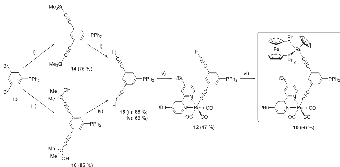
Scheme 3. Synthesis of 10 from 13 : i) \text{HC}\equiv\text{CSiMe}_3 , [(\text{Ph}_3\text{P})_2\text{PdCl}_2]/[\text{CuI}] , \text{HNiPr}_2 , reflux; ii) [n\text{Bu}_4\text{N}]\text{F} , Thf, 25 °C; iii) \text{HC}\equiv\text{CCMe}_2\text{OH} , [(\text{Ph}_3\text{P})_2\text{PdCl}_2]/[\text{CuI}] , \text{HNiPr}_2 , reflux; iv) KOH, toluene, 80 °C; v) 1. \text{LiN}(\text{SiMe}_3)_2 , toluene, 25 °C; 2. [(t\text{Bu}_2\text{bpy})(\text{CO})_3\text{ReCl}] ( 17 ), toluene, reflux; vi) [(\eta^2\text{-dppf})(\eta^5\text{-C}_5\text{H}_5)\text{RuCl}] ( 7 ), [\text{NH}_4]\text{PF}_6 , KOtBu, \text{CH}_2\text{Cl}_2/\text{MeOH} , 25 °C.
