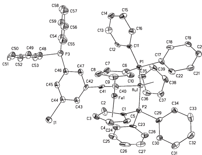
Figure 2. ORTEP drawing of 8 . Thermal ellipsoids are shown at the 50% probability level. The hydrogen atoms are omitted for clarity. Selected bond lengths (Å) and angles (°): Ru1–P1 2.272(2), Ru1–P2 2.267(2), Ru1–D3 1.885(1), Ru1–C40 2.009(9), C40–C41 1.198(11), C41–C42 1.455(12), C44–I1 2.102(13), Fe1–D1 1.637(4), Fe1–D2 1.643(4); P1–Ru1–P2 96.90(8), Ru1–C40–C41 168.5(7), C40–C41–C42 174.9(8), C46–P3–C48 102.0(7), C46–P3–C54 102.9(8), C48–P3–C54 103.9(7) (D1 = centroid of C1–C5; D2 = centroid of C6–C10; D3 = centroid of C35–C39).
