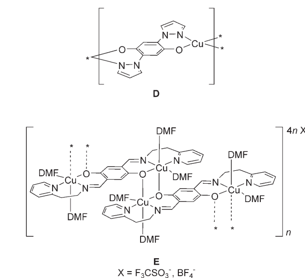
Figure 2. Heisenberg ( S = 1/2 ) spin chains D from ligand A and polymeric S = 1/2 spin dimer system E from ligand B .
