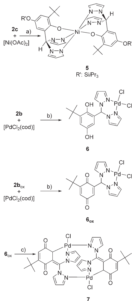
Scheme 2. Synthesis of the Ni II and Pd II complexes 5 , 6 and 6 ox . Formation of macrocyclic dinuclear Pd II complex 7 by deprotonation of 6 ox . Reagents and conditions: a) NaOMe, MeOH, RT; b) CH 3 CN, RT; c) NEt 3 , CH 3 CN, RT
