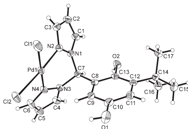
Figure 4. X-ray crystal structure of 6 A (50% probability ellipsoids). Selected bond lengths [Å], bond angles [°], torsion angles [°] and dihedral angles [°]: Pd1–Cl1 2.283(1), Pd1–Cl2 2.295(1), Pd1–N2 2.024(3), Pd1–N4 2.020(3), O1–C10 1.368(4), O2–C13 1.396(3), N1–C7 1.456(4), N3–C7 1.461(4); Cl1–Pd1–Cl2 90.2(1), Cl1–Pd1–N2 90.5(1), Cl1–Pd1–N4 179.5(1), N2–Pd1–N4 89.3(1), N2–Pd1–Cl2 175.6(1), N4–Pd1–Cl2 90.0(1); N2–N1–C7–C8 −69.6(4), N4–N3–C7–C8 76.8(4); Cl1–Pd1–Cl2//N2–Pd1–N4 4.4, N1pz//N3pz 49.0.
