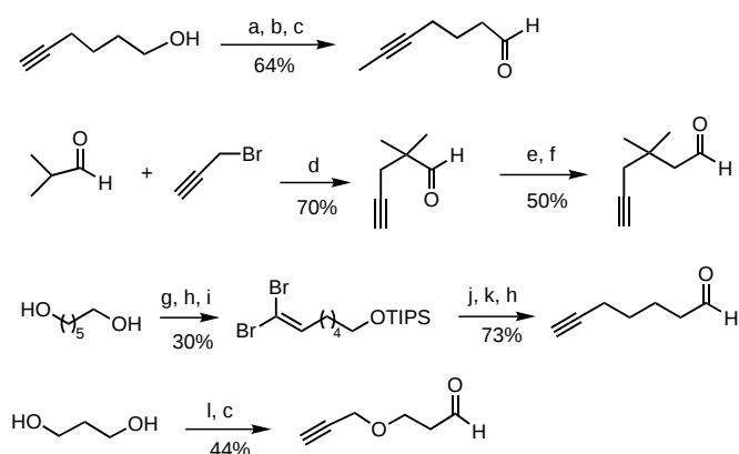
Scheme 10. a) TMSCl, imidazole, \text{CH}_2\text{Cl}_2 , RT; b) 1) n\text{BuLi} , THF, -78^\circ\text{C} , 2) MeI; c) PCC, Celite, \text{CH}_2\text{Cl}_2 , RT; d) \text{NaOH}/\text{H}_2\text{O} , n\text{Bu}_4\text{N}^+\text{I}^- , \text{CH}_2\text{Cl}_2 , DMSO, RT; e) \text{Ph}_3\text{P}=\text{CHOMe} , \text{Et}_2\text{O} , 0^\circ\text{C} ; f) HCl, THF, RT; g) NaH, TIPSCl, THF, RT; h) (\text{COCl})_2 , DMSO, \text{CH}_2\text{Cl}_2 , -78^\circ\text{C} ; \text{Et}_3\text{N} , RT; i) \text{PPh}_3 , \text{CBr}_4 , \text{CH}_2\text{Cl}_2 , RT; j) n\text{BuLi} , THF, 0^\circ\text{C} ; k) 5 M HCl, MeOH, RT; l) NaOH, propargyl bromide, RT.
