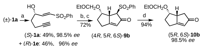
Scheme 7. Application to the enantioselective synthesis of endo 6-oxygenated bicyclo[3.3.0]octenones. a) Lipase PS, vinyl acetate, molecular sieves (4 Å), toluene, RT; b) ClCH 2 OEt, DIPEA, CH 2 Cl 2 , RT; c) 1) [Co 2 (CO) 8 ], CH 2 Cl 2 , RT; 2) Me 3 NO·2H 2 O, RT; d) Zn, NH 4 Cl, THF/H 2 O, RT.
