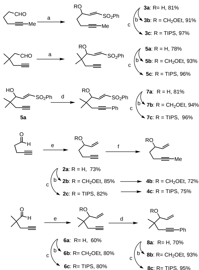
Scheme 3. Synthesis of 1,6-enynes 2–8 . a) \text{PhSO}_2\text{CH}_2\text{SO}_2\text{pTol} , piperidine, \text{CH}_3\text{CN} , 0^\circ\text{C} ; b) \text{ClCH}_2\text{OEt} , DIPEA, \text{CH}_2\text{Cl}_2 , RT; c) TIPSOTf, 2,6-lutidine, \text{CH}_2\text{Cl}_2 , RT; d) 10 mol % \text{Pd}(\text{OAc})_2 , 10 mol % CuI, 20 mol % \text{PPh}_3 , \text{Et}_3\text{N} , PhI, benzene, RT; e) vinylmagnesium bromide, THF, -78^\circ\text{C} ; f) 1) n\text{BuLi} , THF, -78^\circ\text{C} ; 2) MeI, -78^\circ\text{C} .
