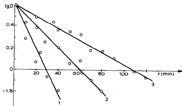
Fig. 1. D^{(330)} vs. time in synthesis of PCA, [\text{Pd}(\text{OAc})_2] = 10^{-4} \text{M} , 1 - P(\text{CO}) = 0.70 \text{ MPa} , 2 - P(\text{CO}) = 0.50 \text{ MPa} , 3 - P(\text{CO}) = 0.25 \text{ MPa} , 40^\circ\text{C} .
