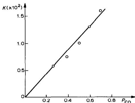
Fig. 2. Rate constant of PCA formation vs. partial pressure of CO, 40°C.
