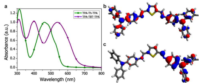
Figure 2. UV-Vis absorption spectrum and computational study of the small molecules. a , Normalized UV-Vis absorption spectrum of TPA-X-TPA small molecules in the solid state. b and c , DFT-calculated (CAM-B3LYP/6-31G*) Kohn-Sham HOMO level for the TPA-Th-TPA molecule: b , Shows the small molecule in the neutral state where the HOMO is delocalized over the entire molecule. c , Protonation of the azomethine nitrogen-atom interrupts conjugation and enforces localization of the HOMO to the non-protonated part of the molecule.
