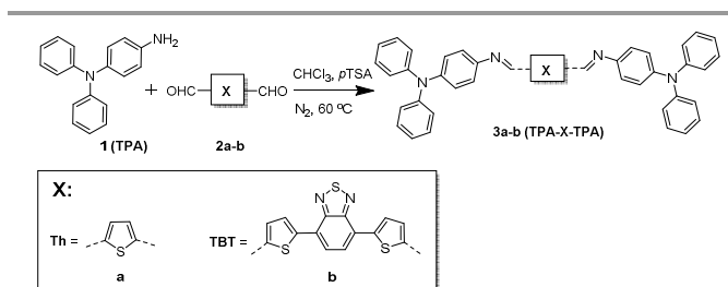
Figure 1. Synthesis and molecular structures of the small-molecule azomethines
