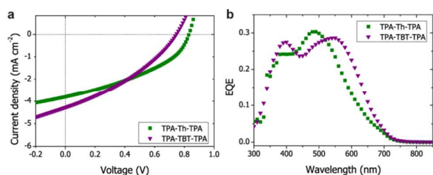
Figure 3. Device performance of small molecule BHJ solar cells. a , J - V characteristics and b , EQE spectra of small molecule bulk heterojunction solar cells based on TPA-X-TPA :[70]PCBM using \text{MoO}_x as hole blocking layer after annealing.
