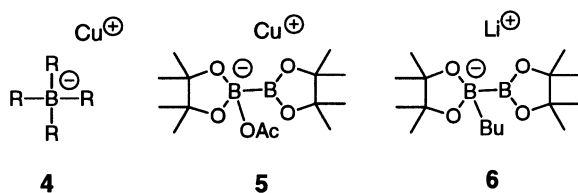
Figure 1. Nucleophilic Boron Species
