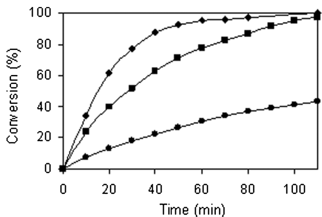
Fig. 6 Oxidation of D-ribose to D-ribonate at (●) 27 (■) 44 and (◆) 50 °C. Reaction conditions: D-ribose (0.1 M, 70 cm 3 ), 5Pd–Bi/C (50 mg), 0.5 L O 2 min -1 , pH 9.
