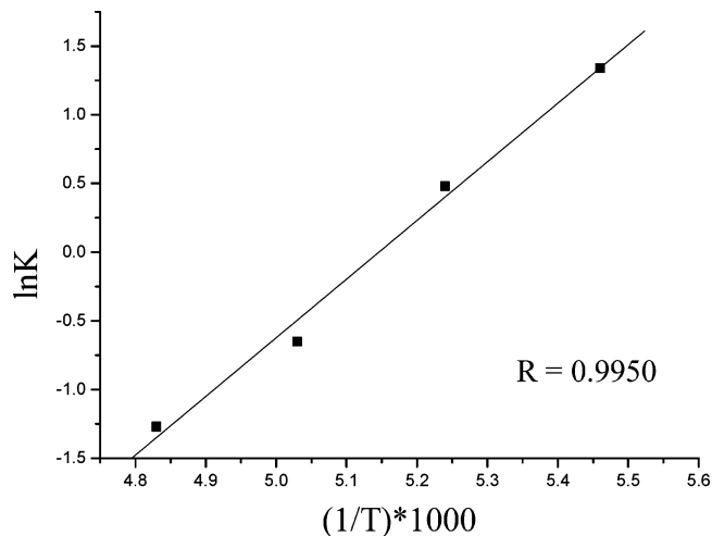
FIGURE 3. Gibbs plot for the equilibrating system 3f + 5a \rightleftharpoons 4f ·OTf − (see the Supporting Information, pp 52–53).
