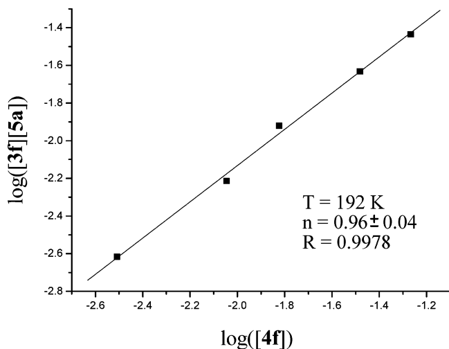
FIGURE 2. Plot of \log([3f] \cdot [5a]) vs \log[4f] for the equilibrating system 3f + 5a \rightleftharpoons 4f ·OTf − at 192 K (see the Supporting Information, pp 52–53).
