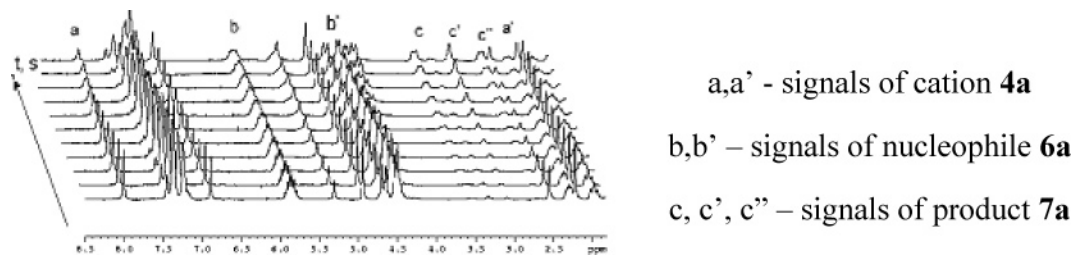
FIGURE 4. Time-dependent proton NMR spectra during the C,C-coupling reaction 4a + 6a → 7a (CD 2 Cl 2 , 200 K, 300 MHz) (see the Supporting Information, pp 17–20).
