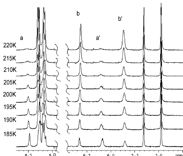
FIGURE 1. Proton NMR spectra of equilibrating system 3f + 5a \rightleftharpoons 4f ·OTf − at various temperatures (CD 2 Cl 2 , 300 MHz). Peaks of cation 4f marked as “a” (H-3) and “a'” (H-4), peaks of starting nitronate 3f marked as “b” (H-3) and “b'” (H-4) (see the Supporting Information, pp 52–53).
