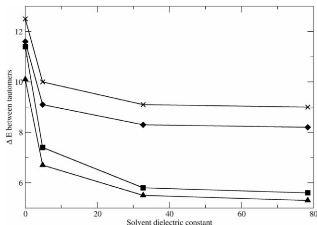
Fig. 6 Energy differences between tautomers in the presence of a continuous solvent dielectric; \times = 7AI, \blacktriangle = 6AI, \blacksquare = 5AI, \blacklozenge = 4-azaindole.
