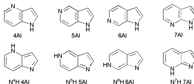
Fig. 1 Azaindole isomers and tautomers explored in this work.
