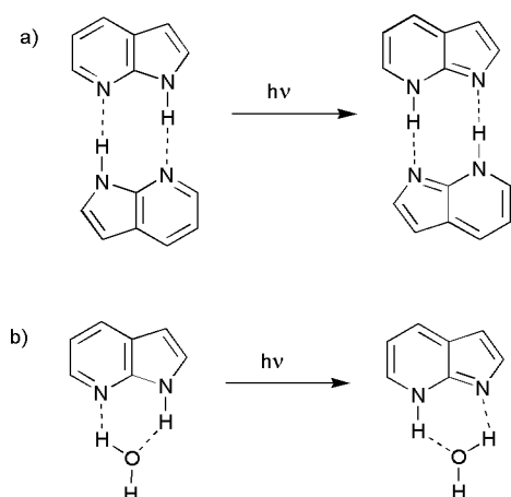
Fig. 3 (a) Excited state double proton transfer of 7-azaindole; (b) excited state proton transfer with one water molecule.
