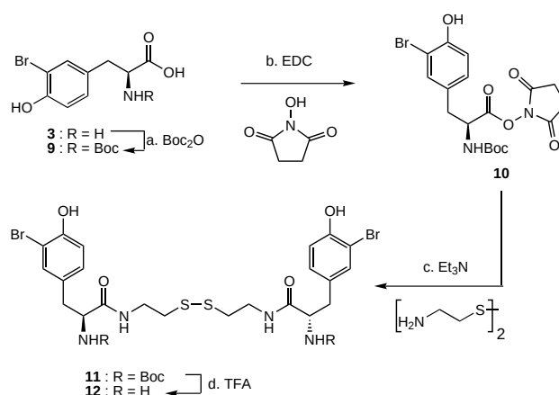
Scheme 2. Synthesis of diamino-psammaplin A ( 12 ). a) di- tert -butyl dicarbonate (2.0 equiv), NaHCO 3 (5.0 equiv), THF/H 2 O 1:1, 23 °C, 12 h; b) NHS (1.9 equiv), EDC (1.7 equiv), 1,4-dioxane, 23 °C, 2 h; c) Et 3 N (2.0 equiv), cystamine · 2 HCl (0.5 equiv), 1,4-dioxane/MeOH 1:1, 23 °C, 12 h, 46 % over three steps; d) TFA (10.0 equiv), CH 2 Cl 2 , 23 °C, 2 h, 95 %.
