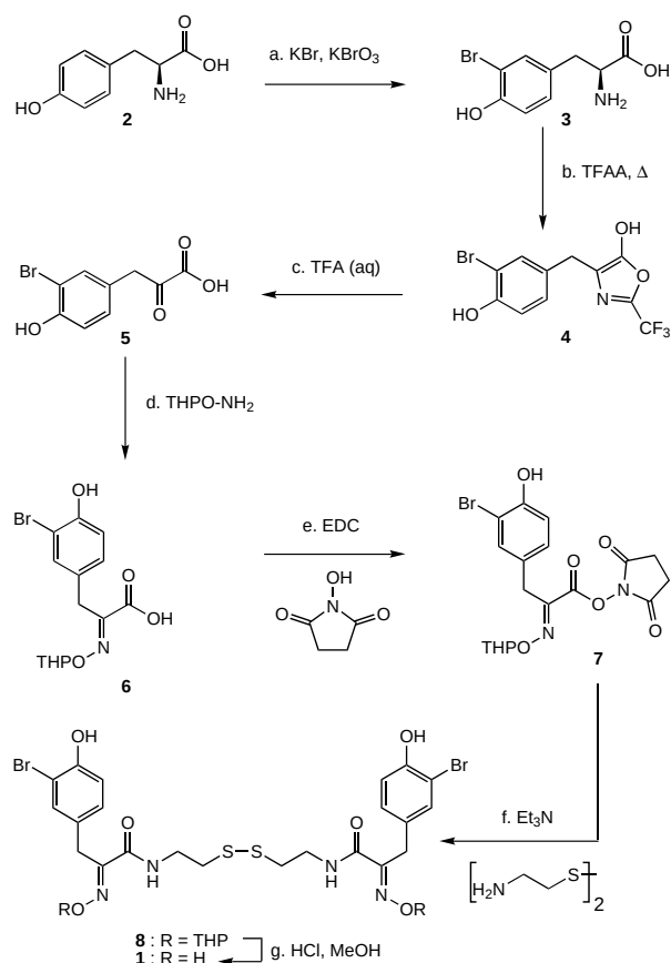
Scheme 1. Total synthesis of psammaplin A ( 1 ) from L-tyrosine ( 2 ). a) KBrO 3 (0.3 equiv), KBr (2.0 equiv), H 2 O (0.25 M HCl), 23 °C, 12 h, 81 %; b) TFAA (excess), 80 °C, 12 h; c) 70 % TFA (aq), 23 °C, 24 h, 60 % over two steps; d) THP-ONH 2 (1.5 equiv), EtOH, 23 °C, 12 h; e) NHS (1.9 equiv), EDC (1.7 equiv), 1,4-dioxane, 23 °C, 2 h; f) Et 3 N (2.0 equiv), cystamine · 2 HCl (0.5 equiv), 1,4-dioxane/MeOH 1:1, 23 °C, 12 h; g) HCl (4.0 equiv), CH 2 Cl 2 /MeOH (20:1), 60 °C, 2 h, 36 % over five steps. EDC = 1-[3-(dimethylamino)propyl]-3-ethylcarbodiimide; NHS = N-hydroxysuccinimide; TFA = trifluoroacetic acid; TFAA = trifluoroacetic anhydride; THP-ONH 2 = O-(tetrahydro-2H-pyran-2-yl)-hydroxylamine.
