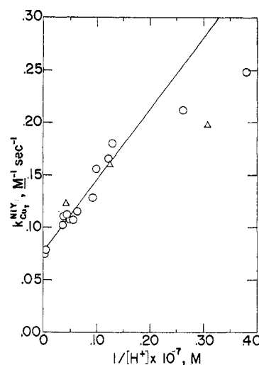
Figure 4.—Resolution of the reaction rate constant, k_{\text{CuT}}^{\text{NiY}} into rate constants for Cu 2+ and CuOH + reaction with NiY -2 : O, 10^{-4} M data; \Delta , 10^{-5} M data.
