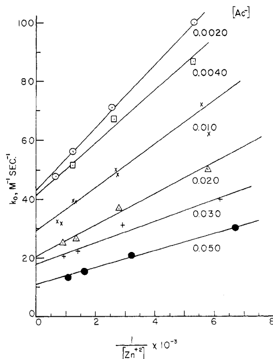
Figure 3.—Effect of acetate ion on the resolution of the observed rate constant into its direct rate constant (intercept = k_{\text{CuT}}^{\text{ZnY}} ) and indirect rate constant (slope = k_{\text{CuT}}^{\text{Y}^-}/K_{\text{ZnY}} ). The molarity of the acetate ion concentration is shown for each series. The copper acetate complexes can be considered not to react with \text{ZnY}^{-2} by comparison to \text{Cu}^{+2} ; pH 5.02, \mu = 0.10 , 25.0^\circ .
