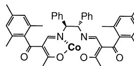
Figure 1. ( S )-MPAC.
