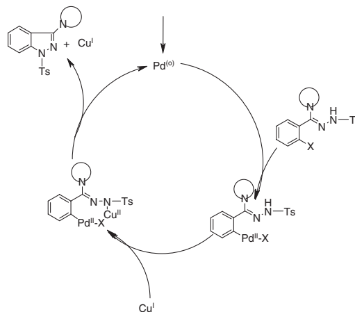
Scheme 3. Plausible mechanism.
