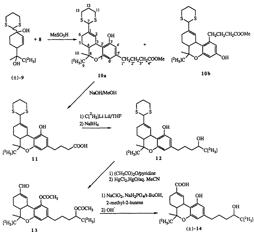
Scheme 2: Preparation of (\pm) -[ ^2\text{H}_6 ]-4''-hydroxy- \Delta^1 -THC-7-oic acid ( 14 )
