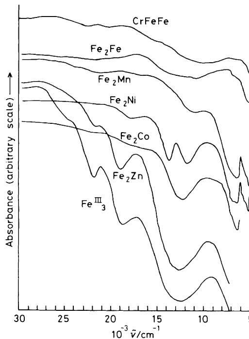
Figure 6. Room-temperature diffuse-reflectance spectra of [\text{Fe}^{\text{III}}_3\text{O}(\text{MeCO}_2)_6(\text{py})_3]\text{Cl} , [\text{Fe}^{\text{III}}_2\text{M}^{\text{II}}\text{O}(\text{MeCO}_2)_6(\text{py})_3]\cdot\text{py} , and [\text{Cr}^{\text{III}}\text{Fe}^{\text{II}}\text{Fe}^{\text{II}}\text{O}(\text{MeCO}_2)_6(\text{py})_3]\cdot\text{py}
