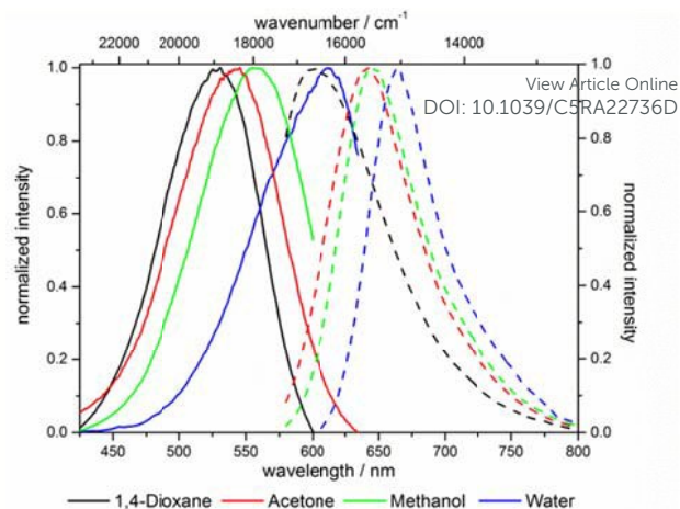
Figure 8. Solvatochromism of 7e .
