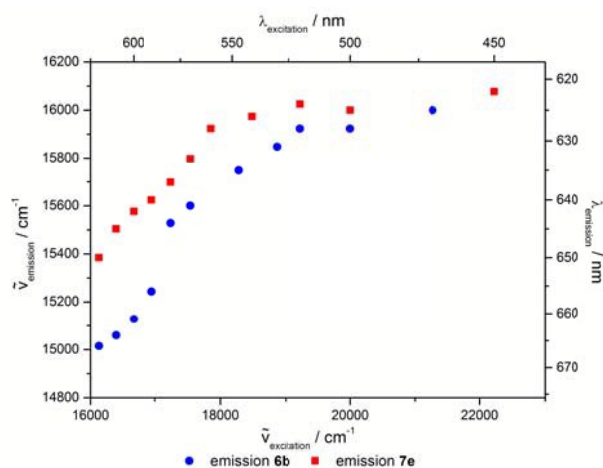
Figure 16. REES of 6b and 7e in acetone.
