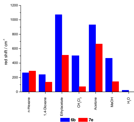
Figure 15. REES of 6b and 7e suspended in different solvents (range of excitation n -hexane: 3333 cm⁻¹, 1,4-dioxane: 2389 cm⁻¹, ethylacetate: 1374 cm⁻¹, CH₂Cl₂: 3607 cm⁻¹, acetone: 3871 cm⁻¹, MeOH: 4127 cm⁻¹, H₂O: 2309 cm⁻¹).
