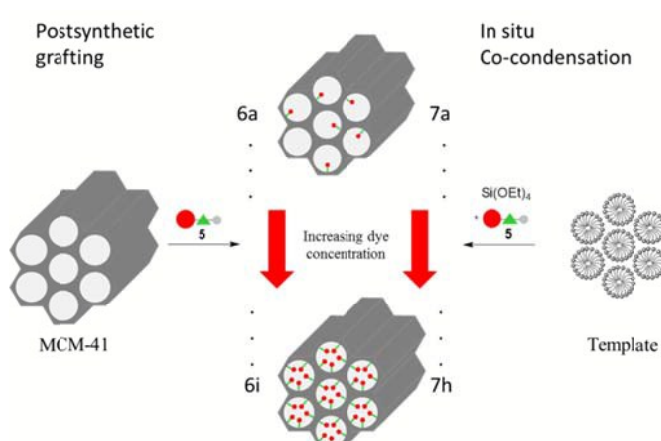
Scheme 2. Synthesis of grafted ( 6a-i ) and co-condensed ( 7a-h ) hybrid materials with different dye loadings.
