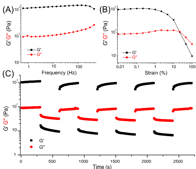
Fig. 5. Oscillatory rheology measurements of Eu(III) gel. (A) Frequency sweeps at 0.1% strain amplitude of the storage modulus G' (■) and loss modulus G'' (●) are shown. (B) The corresponding strain dependence at a f = 1 \text{ Hz} . (C) Recovery test for Eu(III) gel with alternating strain amplitudes of 20% and 0.1% at f = 1 \text{ Hz} .
