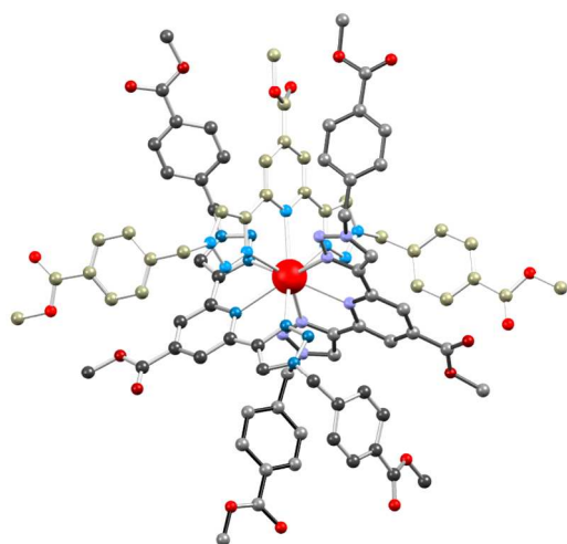
Fig. 2 Ball and stick model of the X-ray crystal structure of Eu13 . Hydrogen atoms and counter-ions are omitted for clarity.
