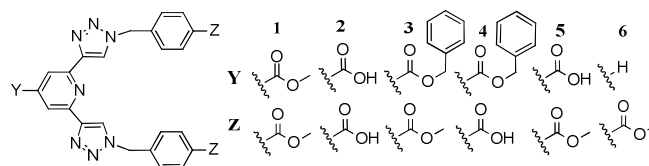
Fig. 1 Btp ligands functionalised at positions Y and Z.
