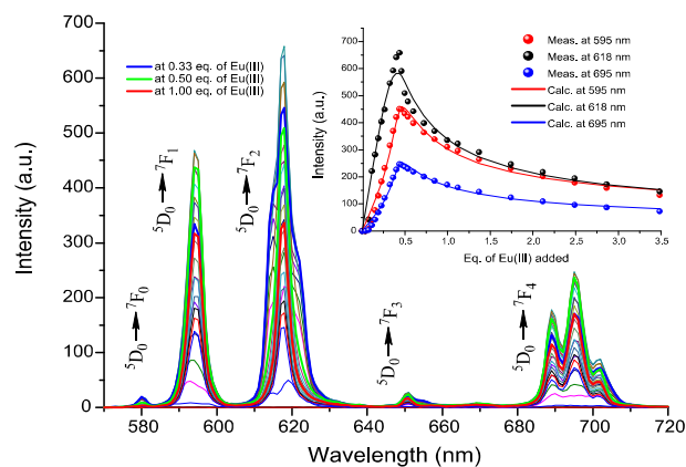
Fig. 3 Changes in \text{Eu(III)} centred luminescence spectra upon titration of 1 in \text{CH}_3\text{CN} ( c = 1 \times 10^{-5} M) against 0 \rightarrow 3.5 eq. of \text{Eu(OTf)}_3 recorded at 25 °C. (Inset) Experimental binding isotherms at band wavelengths. ( \lambda_{\text{ex}} = 325 nm).
