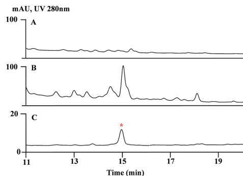
Fig. 3 HPLC analysis of metabolites in strains of Lysobacter enzymogenes OH11. (A) ACL6 in-frame deletion mutant; (B) the ACL6 mutant supplemented with ( R )-3-hydroxy-7-methyloctanoic acyl-SNAC; (C) WAP-8294A2 standard.
