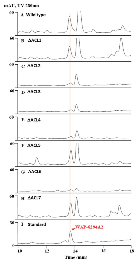
Fig. 2 HPLC analysis of metabolites from various strains of Lysobacter enzymogenes OH11. (A) OH11 wild type; (B–H) disruption mutants of ACL1 through ACL7, respectively; (I) WAP-8294A2 standard. The detection wavelength was 280 nm.
