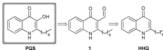
Scheme 1 Synthesis of PQS by Pesci et al. 5 proceeds via HHQ.
