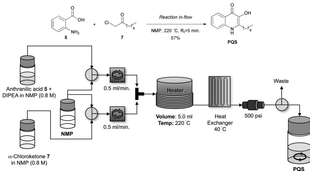
Scheme 4 Schematic of the synthesis of PQS using a Uniqsis FlowSyn™ continuous flow reactor. 22
