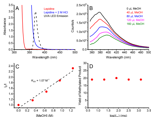
Fig 2 (A) Absorption spectra of lepidine (0.42 M) in MeOH (red), and lepidine (0.42 M) in 2 M HCl in MeOH (blue). When comparing these spectra to the emission profile of the 365 nm LED employed, it becomes evident that lepidine can only be excited in its protonated form under our reaction conditions. (B) Quenching of the emission of lepidine upon increasing concentrations of MeOH in 2M HCl in MeCN. (C) Corresponding Stern-Volmer plot, the slight curvature likely reflects the small special shift in panel B. (D) Yield of methylated lepidine versus the log of the light-on period ( t_{\text{on}} ). For a full description of the experimental procedure and set-up, see ESI.
