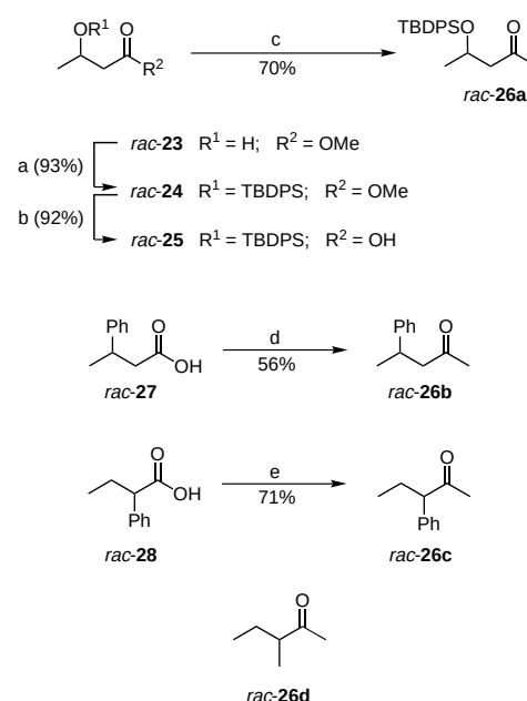
Scheme 5. Synthesis of racemic ketones rac - 26a–d . a) TBDSO, imidazole, THF, RT; b) NaOH, i PrOH/H 2 O, 70 °C; c) MeLi, Et 2 O, −78 °C; d) MeLi, Et 2 O, −78 °C; e) MeLi, Et 2 O, 0 °C.
