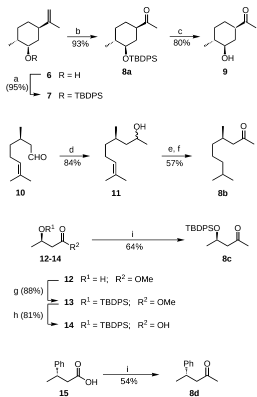
Scheme 2. Synthesis of enantiopure ketones 8a–d . a) TBDPSCl, imidazole, RT; b) \text{O}_3 , \text{CH}_2\text{Cl}_2/\text{MeOH} , -78^\circ\text{C} , \text{PPh}_3 ; c) TBAF, THF, RT; d) \text{MeMgCl} , THF, -78^\circ\text{C} ; e) \text{H}_2 , Pd/C, MeOH, 71 %; f) Dess–Martin periodinane, \text{CH}_2\text{Cl}_2 , RT, 80 %; g) TBDPSCl, imidazole, THF, RT; h) NaOH, i\text{PrOH}/\text{H}_2\text{O} , 70^\circ\text{C} ; i) MeLi, \text{Et}_2\text{O} , -78^\circ\text{C} .
