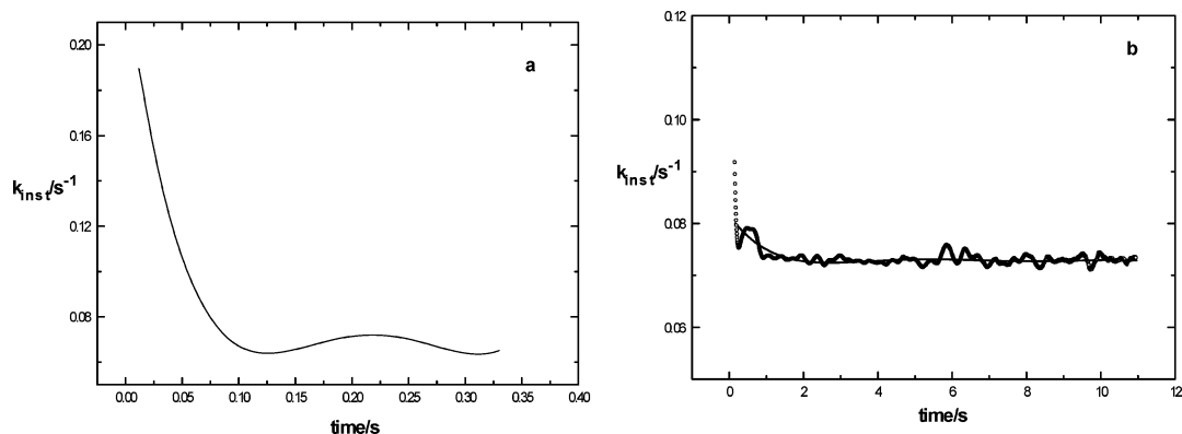
FIGURE 5. IRC time profiles for the reaction of \text{TMT}^+ (0.02 mM) with sodium acetate (0.50 M) in acetic acid. Data for the first 3% of the reaction (a) and that over the first half-life (b).
