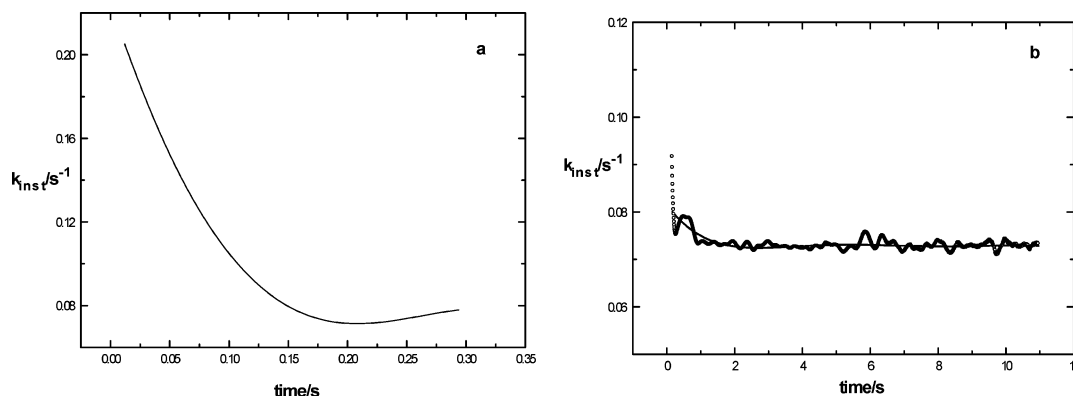
FIGURE 4. IRC time profiles for the reaction of \text{TMT}^+ (0.02 mM) with sodium acetate (0.50 M) in acetic acid. Data for the first 3% of the reaction (a) and that over the first-half-life (b).
