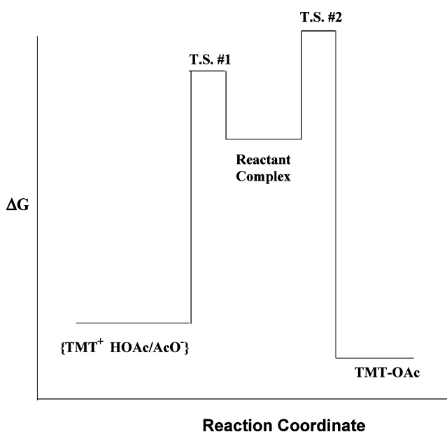
SCHEME 7. Winstein Solvolysis Scheme
