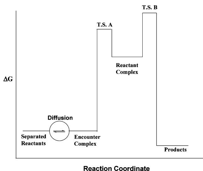
SCHEME 5. Reaction Coordinate Diagram for the Pre-association Mechanism
