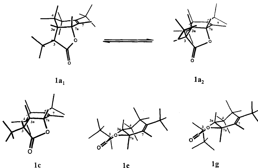
Fig. 2. Conformations of 3a,4,5,7a-tetrahydro-3,6-dimethylbenzofuran-2(3H)-one enantiomers 1a (3 S ,3a S ,7a R ), 1c (3 R ,3a S ,7a R ), 1e (3 S ,3a S ,7a S ), and 1g (3 R ,3a S ,7a S ). Dihedral angle H–C(3a)/H ax –C(4): 75° ( 1a 1 ), 170° ( 1a 2 ), 170° ( 1c ), 180° ( 1e , 1g ); dihedral angle H–C(3a)/H–C(7a): 30° ( 1a 1 ), 28° ( 1a 2 ), 27° ( 1c ), 167° ( 1e , 1g ); dihedral angle H–C(7a)/H–C(7): 60° ( 1a 1 ), 60° ( 1a 2 ), 62° ( 1c ), 105° ( 1e , 1g ); dihedral angle H–C(3a)/H–C(3): 155° ( 1a 1 ), 105° ( 1a 2 ), 16° ( 1c ), 152° ( 1e ), 30° ( 1g ).
