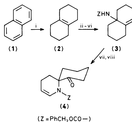
Scheme 1. Reagents: i, Li, EtNH 2 -Me 2 NH (63%) (ref. 4); ii, isopentyl nitrite-HCl (70%) (ref. 5); iii, H 2 -Pt (98%) (ref. 6); iv, NaOMe-MeOH, room temperature, (90%); v, Al-Hg, tetrahydrofuran-H 2 O, reflux (100%) (ref. 7); vi, PhCH 2 OCOCl (99%); vii, O 3 , CH 2 Cl 2 , -78 °C; viii, Me 2 S (43–72%).
