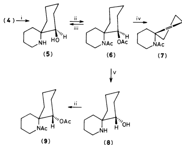
Scheme 2. Reagents: i, \text{H}_2 -Raney Ni, EtOH (93%); ii, \text{Ac}_2\text{O} , \text{Et}_3\text{N} , N,N -dimethylaminopyridine, \text{CH}_2\text{Cl}_2 (94%); iii, \text{K}_2\text{CO}_3 , MeOH (60%); iv, toluene, reflux, 2 days, (96%); v, EtOH ( \text{H}_2\text{O} ), reflux [(6) \rightarrow (9), 87%].
