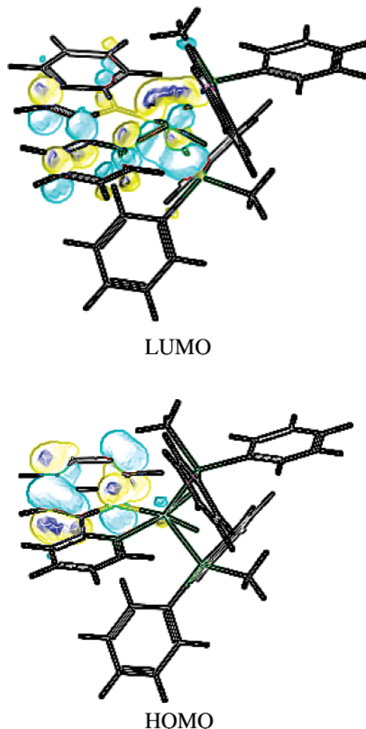
Figure 4. Jaguar representation of the frontier orbitals of 6c , as determined by a DFT calculation.
