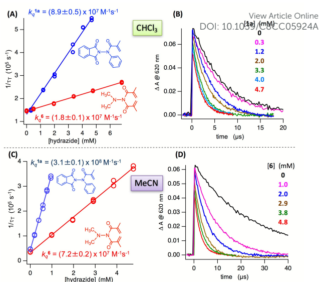
Figure 1. Left: Determination of the bimolecular quenching rate constants k_q for quenching of TX triplet states by acrylanilides using laser flash photolysis ( \lambda_{\text{ex}} = 355 nm, 7 ns pulse width). Inverse TX triplet lifetime from triplet absorption decay traces monitored at 620 nm vs. varying hydrazide concentrations in argon saturated CHCl 3 (A) and MeCN (C) solutions. Right: Transient absorption decay traces of TX triplets different concentrations of 1a and 6 in argon saturated CHCl 3 (B) and MeCN (D) solutions.
