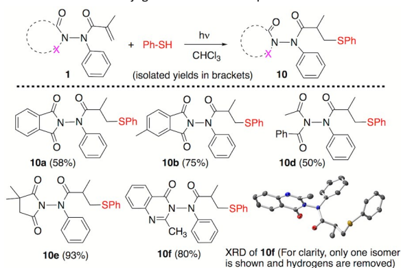
Scheme 5: Excited state conjugate addition of thiophenol to 1.
