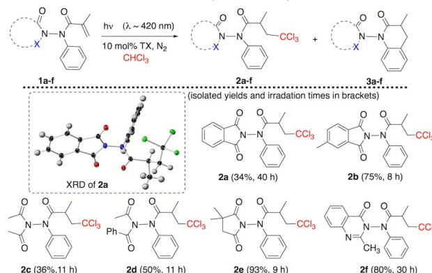
Scheme 2: Excited state chloromethylation of acrylanilides.
