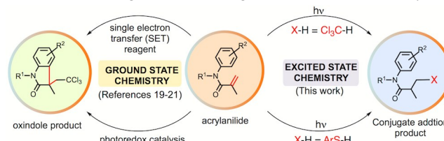
Scheme 1: Contrasting excited state and ground state reactivities of acrylanilides.
