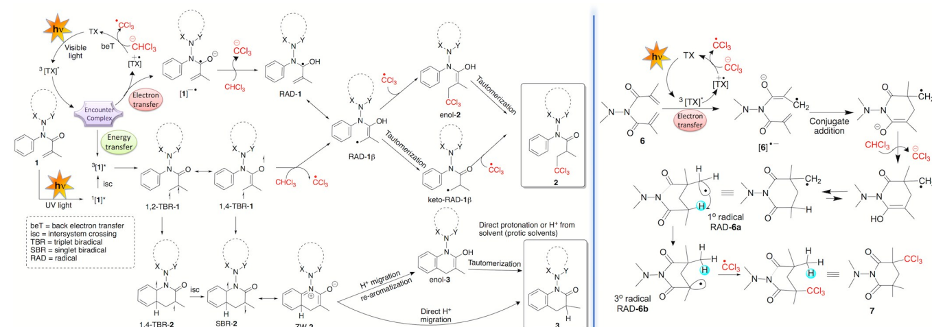
Scheme 4: Mechanistic pathway for chloromethylation of 1a-f .
