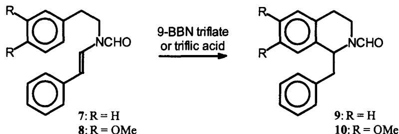
Scheme 2. Synthesis of tetrahydroisoquinolines from N -arylethyl enamides
