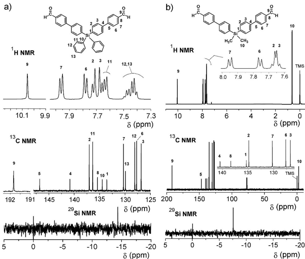
Fig. 4 NMR spectra of the dialdehydes 9 ( \text{DMSO}-d_6 ) (right) and 10 ( \text{CDCl}_3 ) (left).
