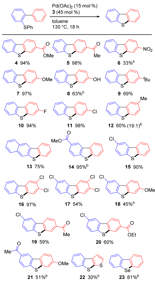
Figure 1 Pd-catalyzed synthesis of dibenzothiophenes via the cleavage of C-H and C-S bonds a
