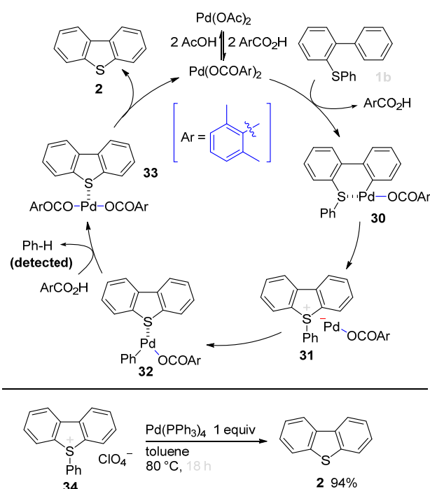
Scheme 4 Possible mechanism
