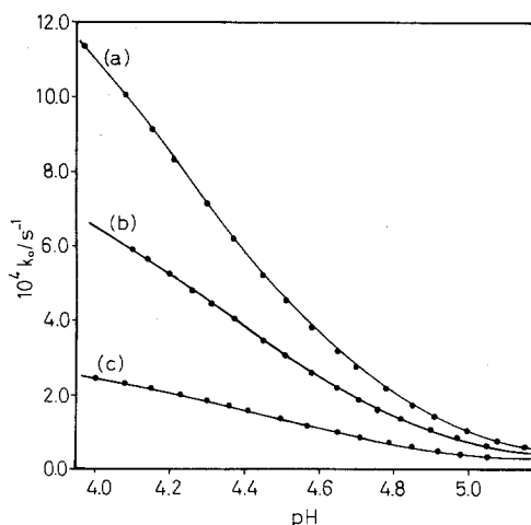
Fig. 4. Effect of pH on the first-order rate constant for the nitrosation of MAN at 25^\circ C , \mu = 0.2 M , [Buf] = 0.120 M and [MAN]/M = (a) 6.07 \cdot 10^{-3} , (b) 3.03 \cdot 10^{-3} , (c) 1.011 \cdot 10^{-3}
