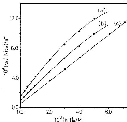
Fig. 5. Influence of the concentration of nitrite on the initial rate of nitrosation of PIP at 25 °C, \mu = 0.2\text{ M} , pH = 4.97 , [PIP]_0 = 9.12 \cdot 10^{-3}\text{ M} and [Buf]/M = (a) 1.00 \cdot 10^{-2} , (b) 4.26 \cdot 10^{-3} , (c) 0.00
