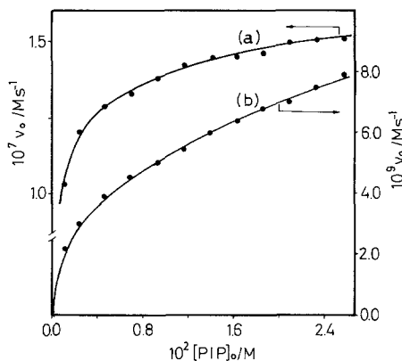
Fig. 7. Influence of the concentration of PIP on the initial rate of formation of NPIP at 25°C, \mu = 0.2 M , [Buf] = 5.02 \cdot 10^{-2} M , pH = 4.96 and [Nit]_0 / M = (a) 5.12 \cdot 10^{-3} , (b) 5.46 \cdot 10^{-4}
