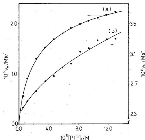
Fig. 6. Influence of the concentration of PIP on the initial rate of formation of NPIP at 25 °C, \mu = 0.2\text{ M} , [Nit]_0 = 1.09 \cdot 10^{-3}\text{ M} , pH = 4.98 and [Buf]/M = (a) 8.50 \cdot 10^{-2} , (b) 4.12 \cdot 10^{-3}
