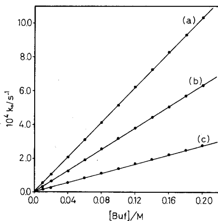
Fig. 2. Influence of the concentration of acetate buffer on the first-order rate constant for the nitrosation of MAN at 25 °C, \mu = 0.2\text{ M} , pH = 4.37 and [MAN]/M = (a) 6.07 \cdot 10^{-3} , (b) 3.03 \cdot 10^{-3} , (c) 1.011 \cdot 10^{-3}
