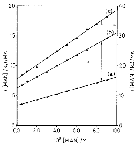
Fig. 3. Influence of the concentration of MAN on the first-order rate constant for the formation of NMAN at 25 °C, \mu = 0.2\text{ M} , pH = 4.37 and [Buf]/M = (a) 0.200 , (b) 0.100 , (c) 0.040
