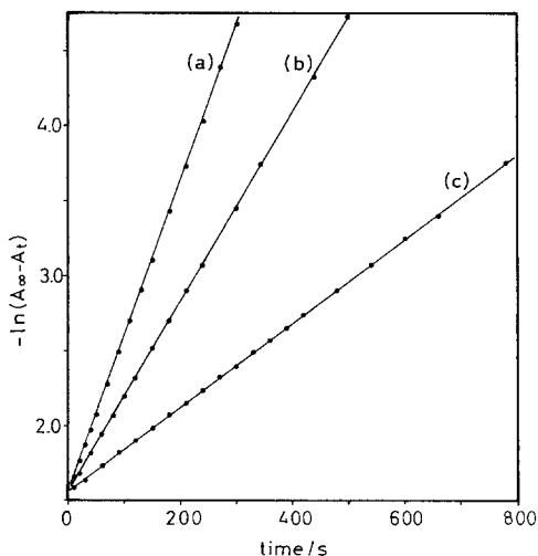
Fig. 1. Typical first-order plots for the nitrosation of MAN in acetate buffer at 25°C, \mu = 0.2\text{ M} , [\text{Buf}] = 0.200\text{ M} , pH = 4.37 , [\text{MAN}]/M = (a) 6.07 \cdot 10^{-3} , (b) 3.03 \cdot 10^{-3} , (c) 1.011 \cdot 10^{-3} and [\text{Nit}]_0 = 2.94 \cdot 10^{-5}\text{ M}
