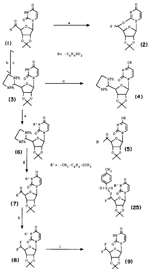
Scheme 1. Reagents: (a) DAST, \text{CH}_2\text{Cl}_2 ; (b) N,N' -diphenylethylenediamine; (c) pTsOH, \text{CH}_3\text{COCH}_3 ; (d) mesitylenesulphonyl chloride, DMAP, DBO, 4- \text{NO}_2 - \text{C}_6\text{H}_4 -OH; (e) NaH, 4-MeO- \text{C}_6\text{H}_4 - \text{CH}_2\text{Cl} ; (f) pTsOH; (g) pTsOH; (h) DAST, \text{CH}_2\text{Cl}_2 ; (i) CAN.
