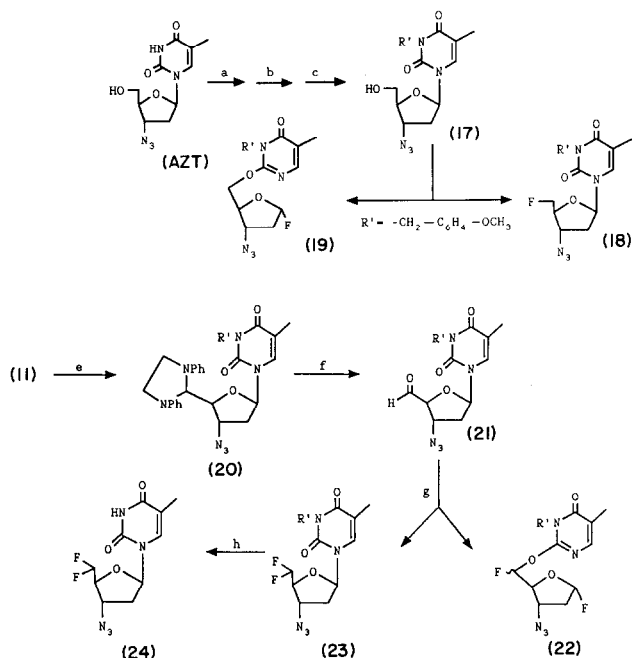
Scheme 3. Reagents: (a) tBDPSCI, C 6 H 5 N; (b) NaH, 4-OMe-C 6 H 4 -CH 2 Cl; (c) TBAF, THF; (d) DAST; (e) NaH, 4-OMe-C 6 H 4 -CH 2 Cl; (f) TsOH; (g) DAST; (h) CAN.
