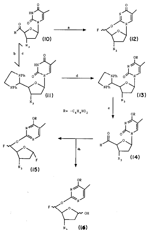
Scheme 2. Reagents: (a) DAST; (b) N,N' -diphenylethylenediamine; (c) TsOH; (d) mesitylene-sulphonyl chloride, DMAP, DBO, 4- \text{NO}_2 - \text{C}_6\text{H}_4 -OH; (e) TsOH.
