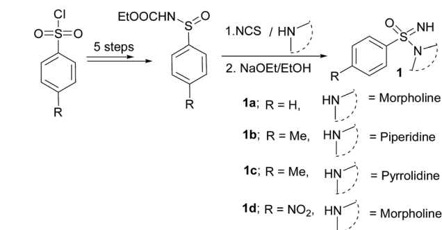
Scheme 1 Synthesis of sulfonimidamides.
